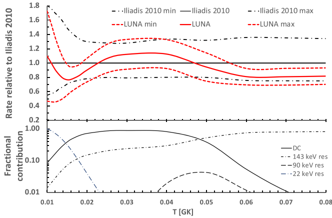
Fig. 3. Top: Reaction rate relative to Iliadis et al. [30]. Bottom: fractional contributions of the individual cross section components to the total rate.
