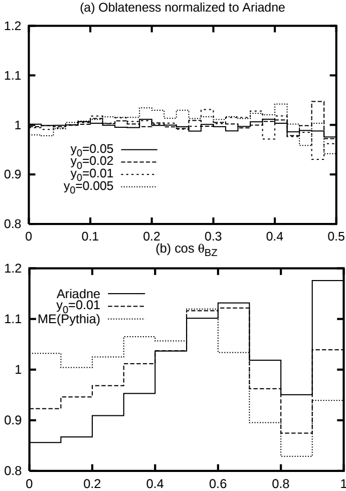
Fig. 1. (a) Ratios of the oblateness event shape on parton level at E_{\text{CM}} = 91 GeV for the new ME matching algorithm using different values of Q_0 w.r.t. to the standard ARIADNE program. The full line is with y_0 = Q_0^2/Q^2 = 0.05 , long-dashed: y_0 = 0.02 , dashed: y_0 = 0.01 and dotted: y_0 = 0.005 . (b) The distribution in the Bengtsson-Zerwas angle on parton level. The full line is standard ARIADNE, the dashed line is the new ME matching algorithm with y_0 = 0.01 and the dotted line is the tree-level \mathcal{O}(\alpha_s^2) ME-only generator in PYTHIA with y_0 = 0.01 .
