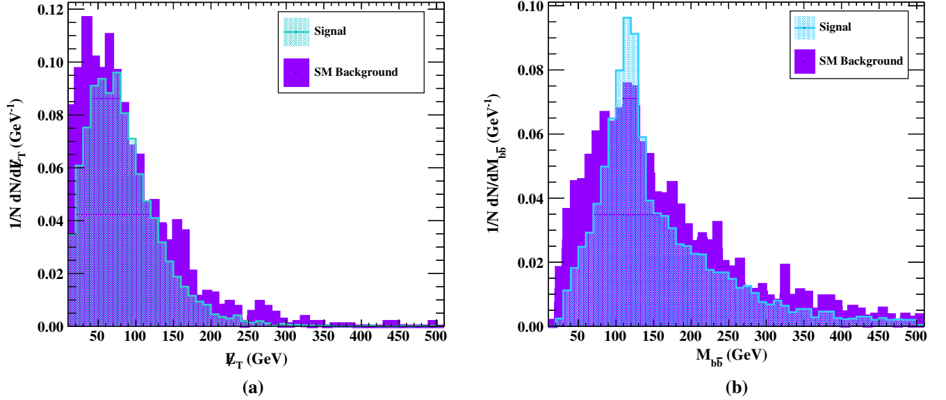
FIG. 6. Normalized distribution of the (left panel) Missing transverse energy ( E_T ) and (right panel) the invariant mass of b\bar{b} pair after the basic kinematical acceptance cuts [Eq. (12)] for the benchmark BP1.
