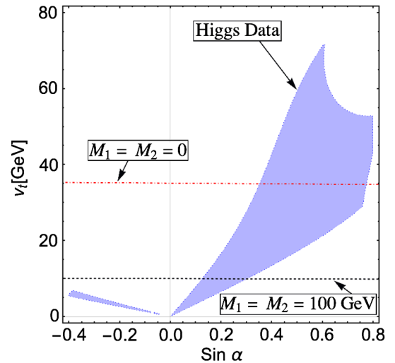
FIG. 2. Model parameter space allowed in the (\sin \alpha - v_t) plane from the latest Higgs data (shaded blue) [34,35] for a benchmark scenario m_3(m_5) = 300(400) GeV allowed by the theoretical constraints. The dot-dashed (red) and dashed (black) lines correspond to the bound coming from theoretical constraint for vanishing and nonvanishing trilinear term of the GM potential, respectively.
