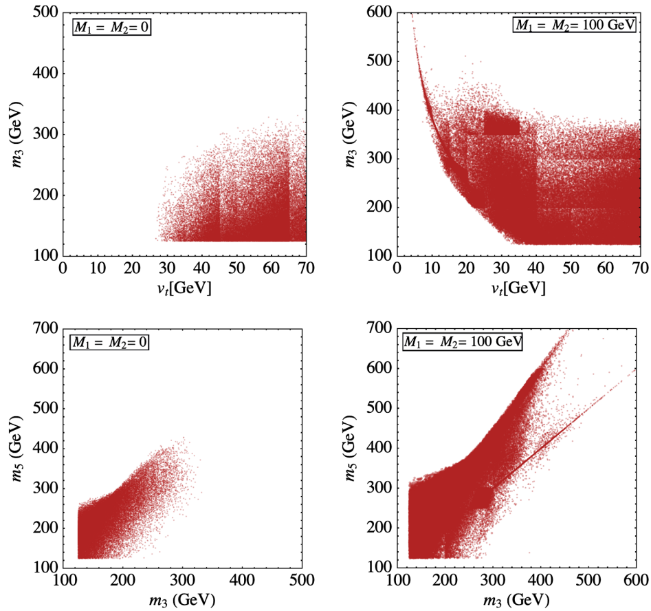
FIG. 1. Allowed regions in the v_t - m_3 plane (upper panel) and in the m_3 - m_5 plane (lower panel) from theoretical constraints for zero (left panel) and nonzero (right panel) trilinear couplings.
