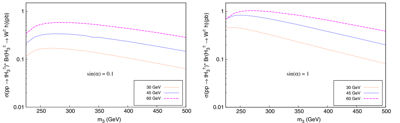
FIG. 5. The production cross section times branching ratio plot for charged Higgs decaying to W^\pm h channel for two values of \sin\alpha = 0.1 (left panel) and \sin\alpha = 1.0 (right panel). The color coding is the same as in Fig. 4.
