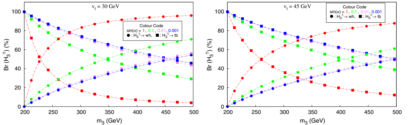
FIG. 3. The branching ratio of charged Higgs H_3^\pm for two different choices of the triplet vev, v_t = 30 GeV (left panel) and v_t = 45 GeV (right panel). The box and circular points define the two distinct decay modes of the charged scalar, H_3^\pm \rightarrow t\bar{b} and H_3^\pm \rightarrow W^\pm h channel respectively while the four different colors (red, green, magenta, blue) corresponds to four different orders of magnitude for \sin \alpha (1,0.1,0.01,0.001).
