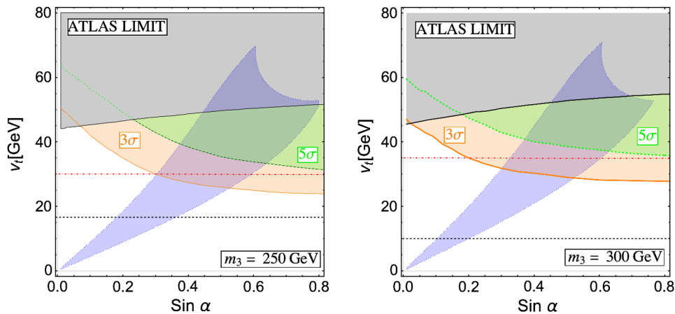
FIG. 7. The combined results on the model parameter space in the (\sin \alpha - v_t) plane for charged Higgs masses m_3 = 250 GeV (left panel) and m_3 = 300 GeV (right panel). The color coding for Higgs data and theoretical constraint is same as in Fig. 2. The gray shaded region with black solid boundary corresponds to the current ATLAS limit from charged Higgs analysis [19]. The green(dashed) and orange(solid) lines are respectively the 5\sigma and 3\sigma signal significance reach at 14 TeV LHC with 3 ab^{-1} luminosity in the charged Higgs decaying to Wh mode.
