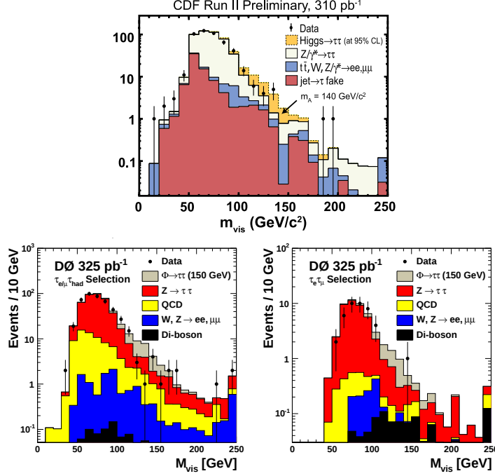
Fig. 5. Distribution of the visible mass M_{\text{vis}} for the analysis by CDF (top), and the two options considered by DØ : the one involving hadronic tau decays (bottom left) and one with the e\mu final state (bottom right). Data are compared to the predicted background from the SM and a possible signal.
