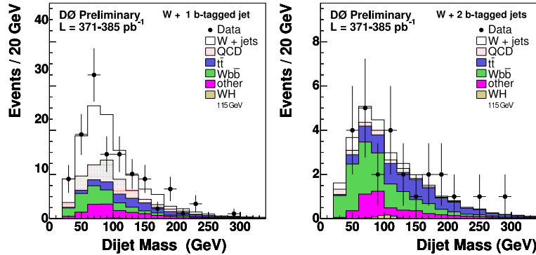
Fig. 1. Dijet invariant mass in the W + 2 jet events having one tagged b -jet (left) or both of them b -tagged (right) in the Higgs search by the DØ Collaboration. Data (crosses) are compared to the background predictions (stacked histograms).
