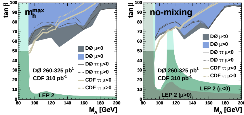
Fig. 6. Region, which is excluded at 95% C.L. by the ditau and four-b searches of the MSSM neutral Higgs boson by the DØ Collaboration, in the (M_A, \tan \beta) plane for the m_h^{\max} (left plot) and the no-mixing scenario (right plot) for \mu = +0.2 TeV and \mu = -0.2 TeV and assuming a mass of the top quark of 172.7 \text{ GeV}/c^2 . The LEP limits extrapolated to the region \tan \beta > 50 and those by the ditau channel by CDF are also shown.
