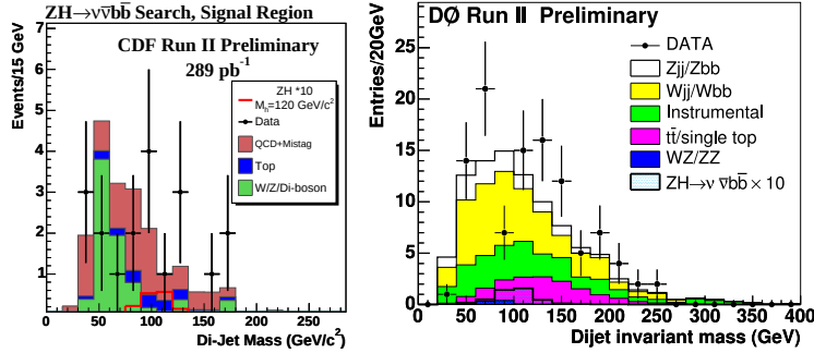
Fig. 2. Dijet Invariant mass distributions for the final selection in the CDF (left) and DØ (right) analyses searching for ZH \rightarrow \nu\bar{\nu}b\bar{b} . Data is in both cases compared to the predicted backgrounds before setting the cuts on the dijet mass to increase the sensitivity to the signal.
