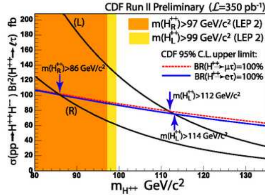
Fig. 8. 95% C.L. curves for p\bar{p} \rightarrow H^{++}H^{--} \rightarrow l^+\tau^+l^-\tau^- . The arrows show the limits for the two analysis, Excluded values by the LEP experiments for the Higgs mass are shown as the coloured region.
