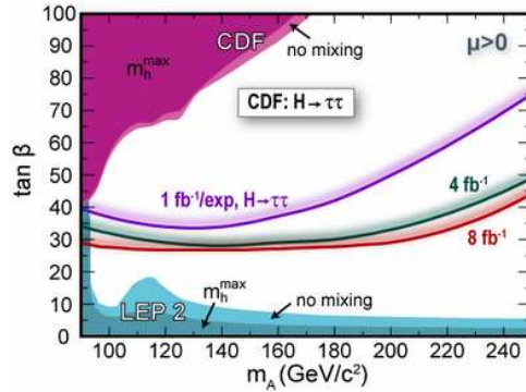
Fig. 7. Excluded regions in the (M_A, \tan \beta) plane for the m_h^{\max} and the no-mixing scenario with \mu > 0 and the expectations for increased integrated luminosity samples.
