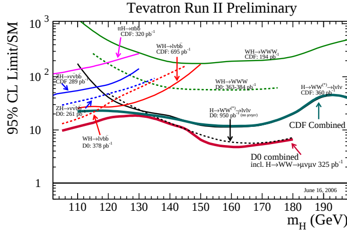
Fig. 3. Cross section limits for Higgs production at Tevatron in Run II as a function of the Higgs mass. The limit is represented in units of the predicted cross section in the SM. Limits are shown individually for each analysis and in the combination performed inside each experiment.
