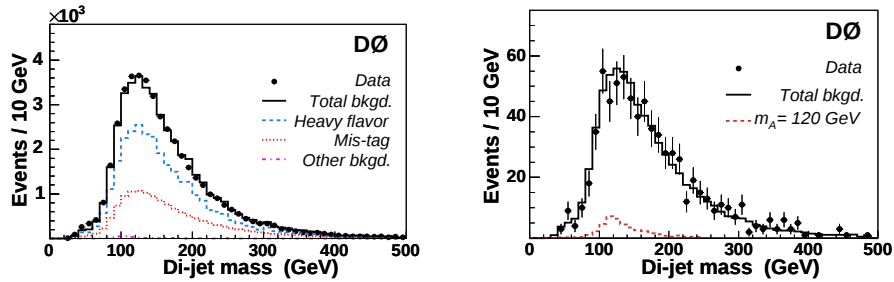
Fig. 4. On the left-hand plot, fit of the invariant mass spectrum of the two leading jets in the sample containing two tagged b -jets to the sum of the backgrounds. On the right-hand plot, invariant mass distribution of the two leading jets in events with at least three tagged b -jets, compared to the estimated background and the Higgs-boson signal that can be excluded at 95% C.L.
