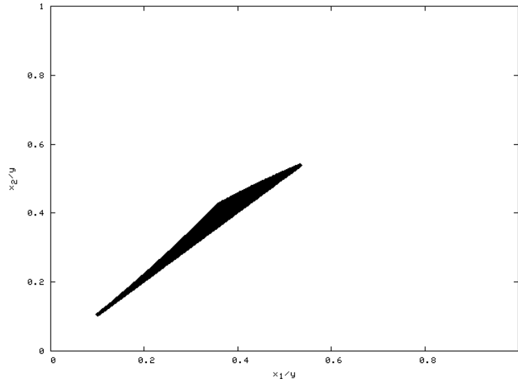
Figure 3.1: Polarizations which make V_4 stable.
