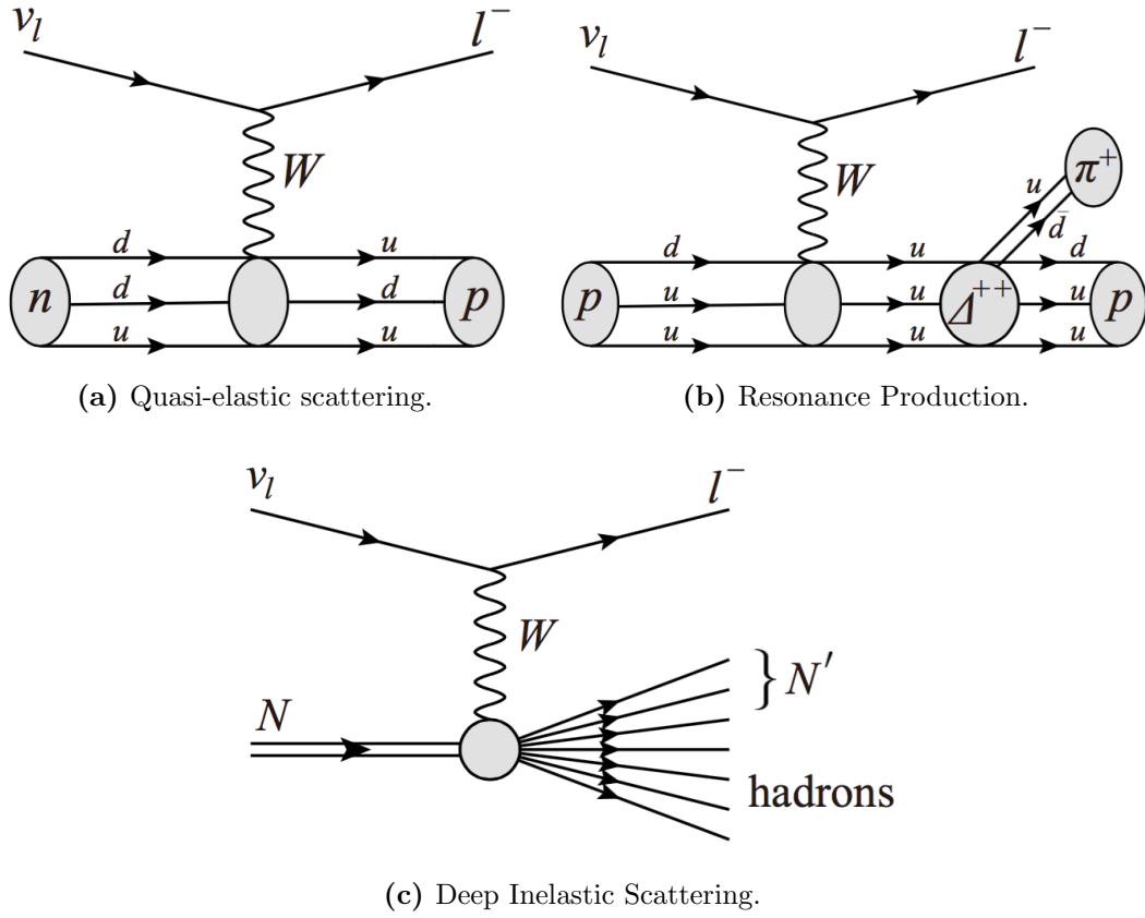
Figure 1.6: Feynman diagram of charged current neutrino-nucleus scattering.
