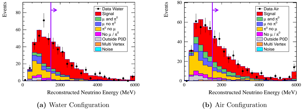
Figure 4.9: The N-1 plot of the neutrino energy selection cut for the water and air configuration. The plots are area-normalized to emphasize shape differences between the data and MC. The last bin contains the overflow bin. The cut value is set at 1.5 GeV for both water and air configuration.
