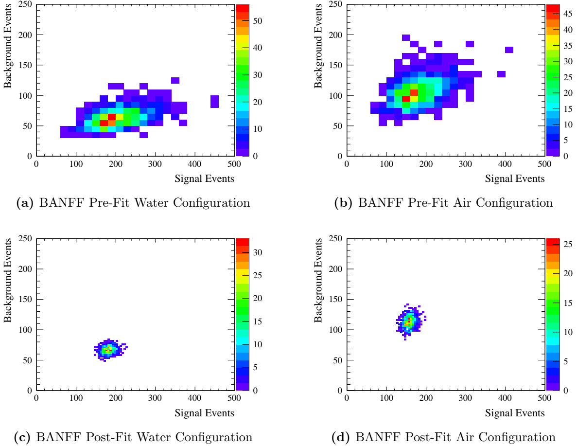
Figure 4.41: Selected number of signal vs background events varied within the BANFF pre- and post-fit flux and cross section systematic uncertainties for the PØD water and air configuration.
