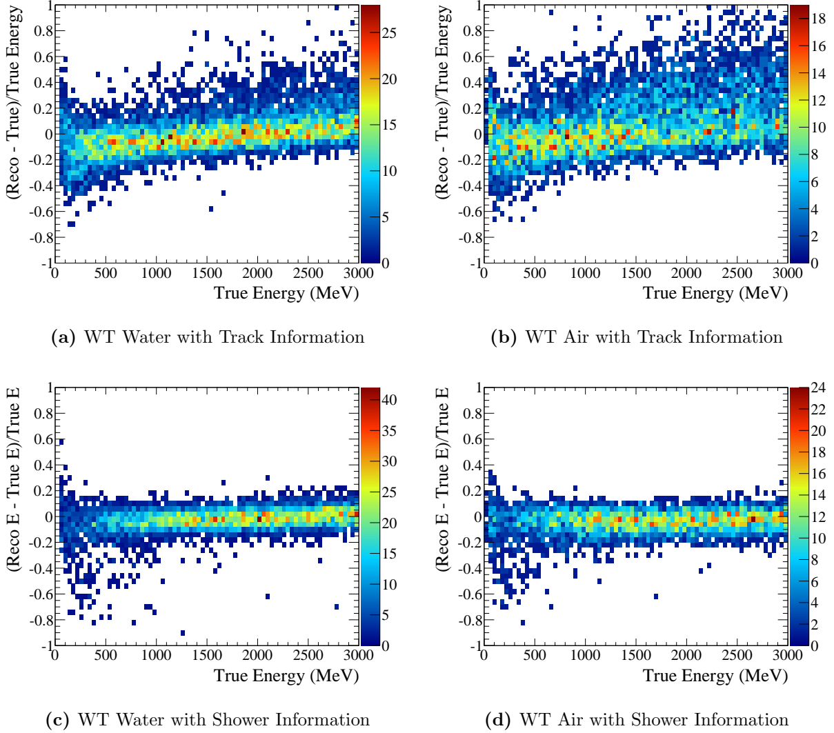
Figure 3.8: Relative reconstructed electron energy to true energy, for Water/Air WT configuration with track and shower reconstruction.
