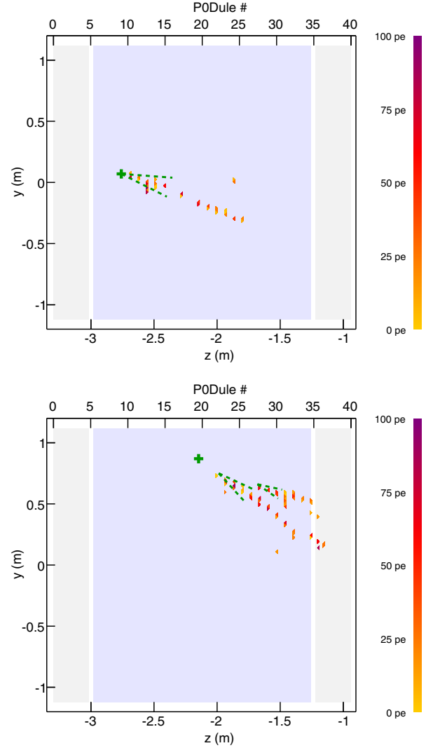
FIG. 1 (color online). Side view of a \text{CC}\nu_e event (top) and a \pi^0 background event (bottom) reconstructed in the PØD. Triangles are hits colored by the charge deposited, the green cross symbol shows the reconstructed shower vertex, and the green dashed lines show the cones of reconstructed showers.
