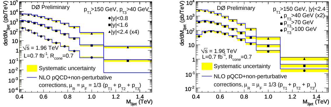
Figure 1: a) Three-jet mass cross section in regions of jet rapidities. The |y| < 2.4 region is scaled by a factor of 4 for readability. Systematic uncertainty is shown by shaded band. Full lines correspond to the NLO calculations with NLOJET++ and MSTW2008 PDFs. No events are found in the highest M_{3\text{jet}} bin in |y| < 0.8 region. b) Three-jet mass cross section in regions of the third jet transverse momenta. The p_{T3} > 40 GeV region is scaled by a factor of 2 for readability. Systematic uncertainty in all three-jet mass bins is shown by shaded band. Full lines correspond to the NLO calculations with NLOJET++ and MSTW2008 PDFs. In both figures, the dataset corresponds to an integrated luminosity of 0.7 \text{ fb}^{-1} .
