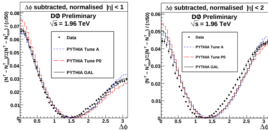
Figure 4: The normalized distribution of \Delta\phi to the leading track in the same minimum bias vertex, for (a) |\eta| < 1.0 and (b) |\eta| < 2.0 . Error bars include systematic uncertainties.
