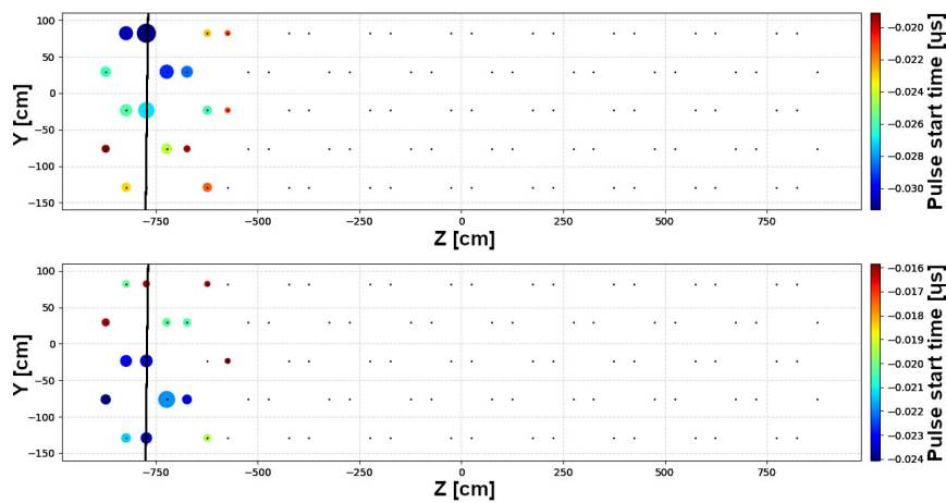
Figure 4. Graphic representation of a cosmic ray passing through the detector and seen by the two facing PMTs walls. The arrival times and and the number of photons to the surface of each PMT are coded through the color and size of the light spot.
