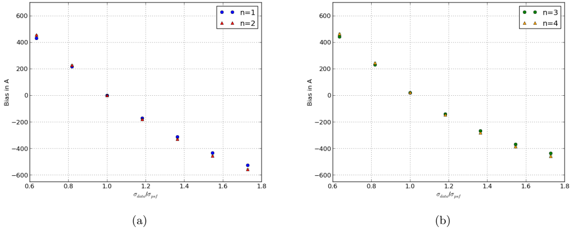
Fig. 12.— Figure 12a shows the bias in A as a function of the ratio of standard deviations \sigma_{\text{data}} and \sigma_{\text{psf}} for the n = 1 and n = 2 cases with the Poisson fit. Figure 12b shows the same for the n = 3 and n = 4 cases. At unity in both figures, the bias in A is approximately zero. Figures were generated using the true value of B and NTRIALS=10,000.
