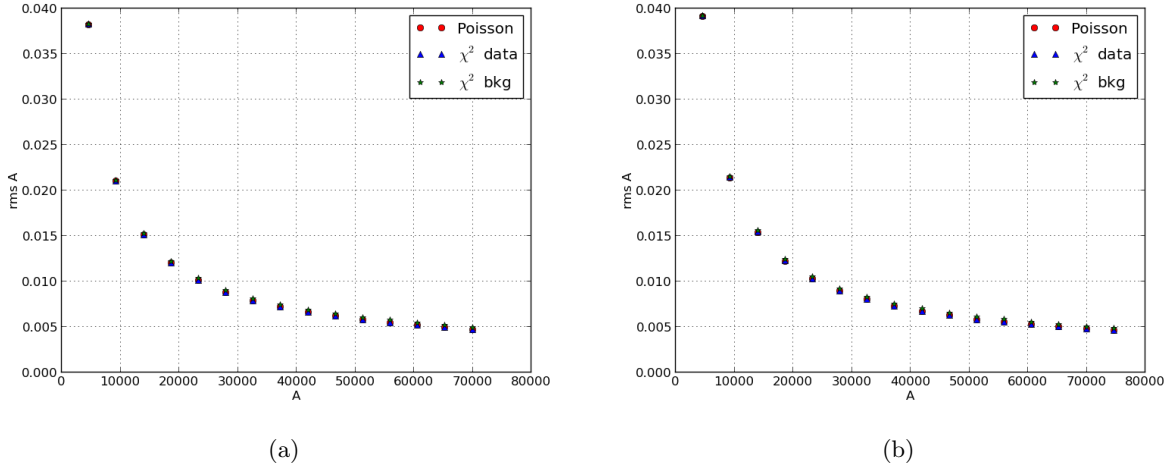
Fig. 6.— Figure 6a shows the normalized RMS of A as a function of A for the n = 1 case; Figure 6b shows the same for the n = 2 case. Fits were constructed with NTRIALS=10,000 and using the true value of B .
