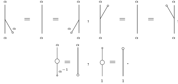
Figure 3.3 – The antipode properties
