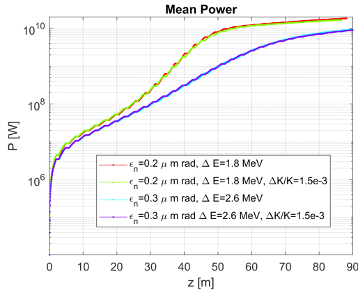
Figure 2: Output of FEL simulations: mean power along the undulator beamline corresponding to different electron beam transverse normalized emittance \epsilon_n and energy spread \Delta E . The curves have been obtained averaging on 50 SASE pulses. Simulations with and without errors in the K parameters of the undulator have been performed.
