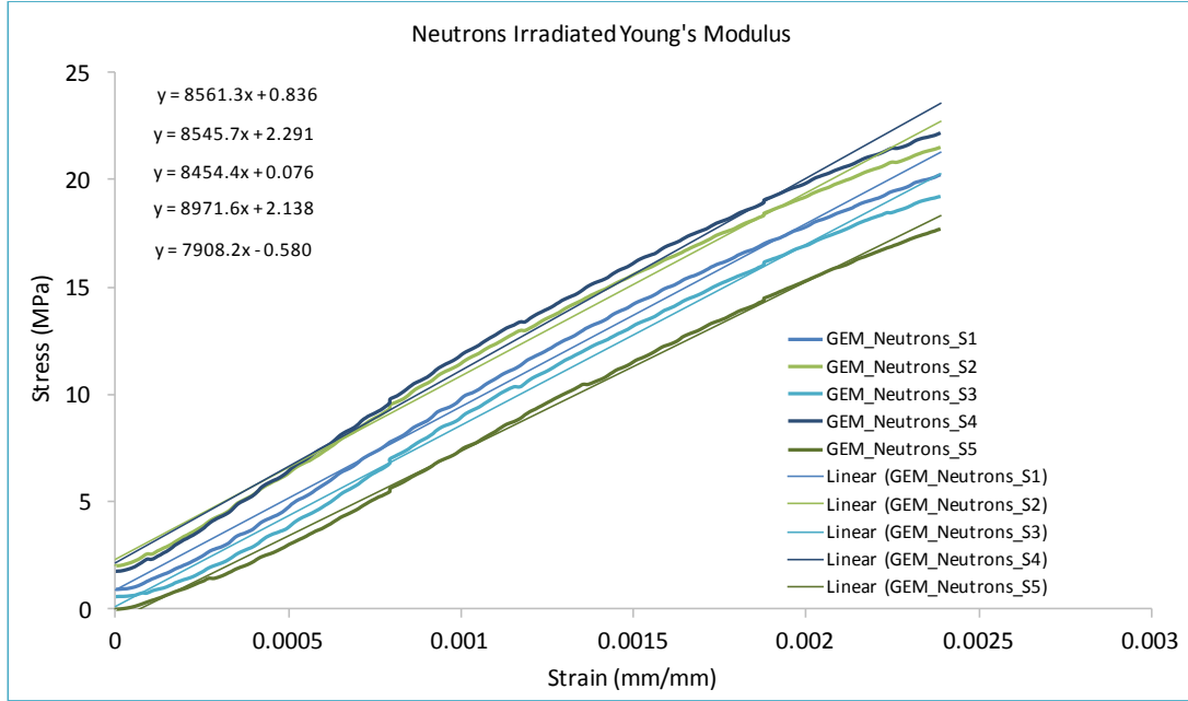
Figure 8. Young's modulus estimation of the neutrons irradiated GEM foil.
