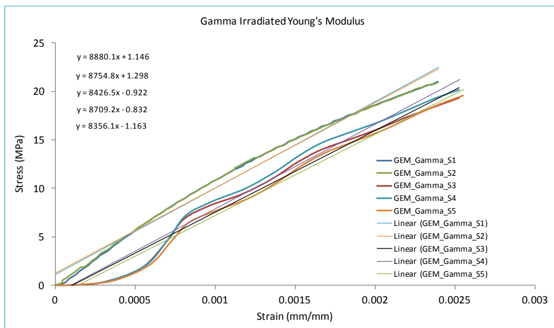
Figure 7. Young's modulus estimation of the gamma irradiated GEM foil.
