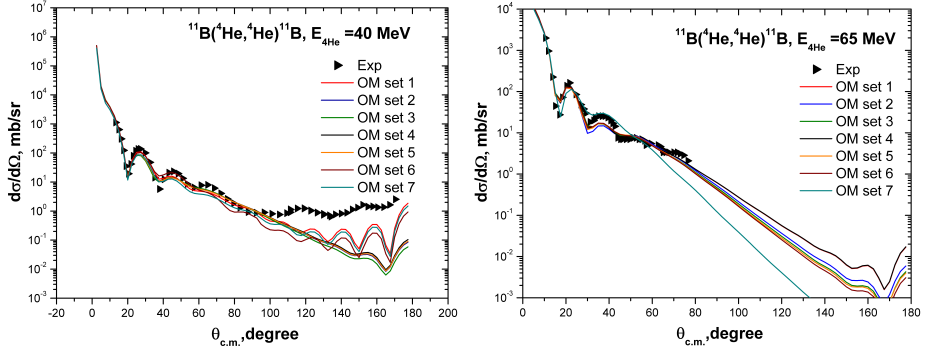
Fig. 1. Solid curves — calculations for the OM of the nucleus with potentials 1–7.
