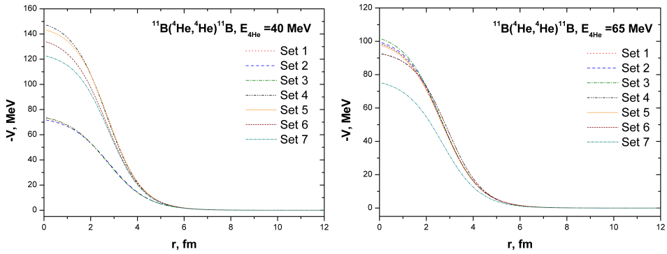
Fig. 2. Radial dependences of the real ( V(r) ) and imaginary ( W_D(r) ) parts of the potentials from Table I.
