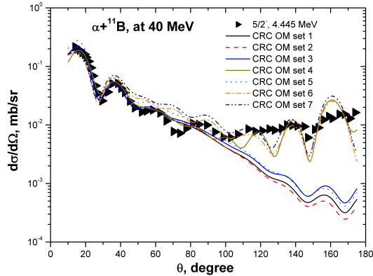
Fig. 4. Solid curves — calculations for the CRC of the nucleus with potentials 1–7.
