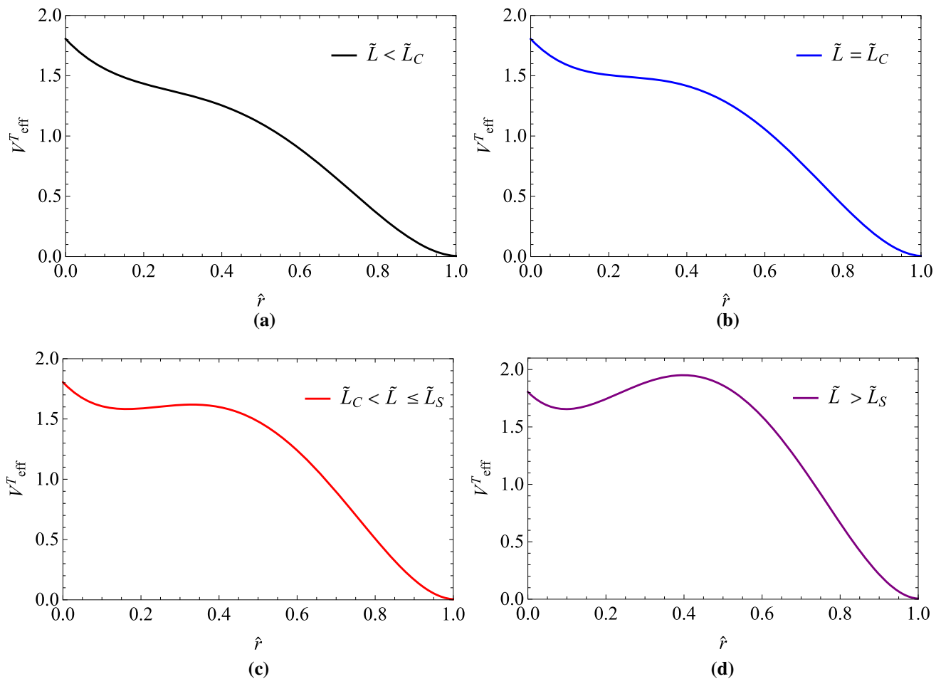
Fig. 1 Variation of effective potential V_{eff}^T(\hat{r}) for timelike geodesics as a function of radial coordinate \hat{r} for different values of angular momentum a \tilde{L} = 2.2 , b \tilde{L} = 2.5 , c \tilde{L} = 2.8 and d \tilde{L} = 3.3 . Here we fix the TWH parameter \gamma_+ to 0.9
