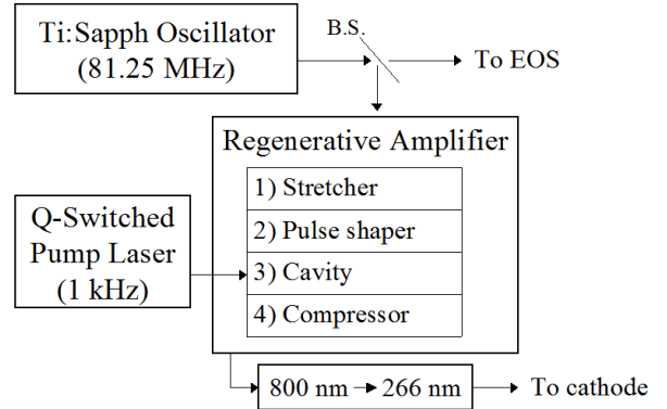
Figure 1: Schematic optical layout with Ti:sapph running as both photoinjector drive laser and EOS probe laser.
