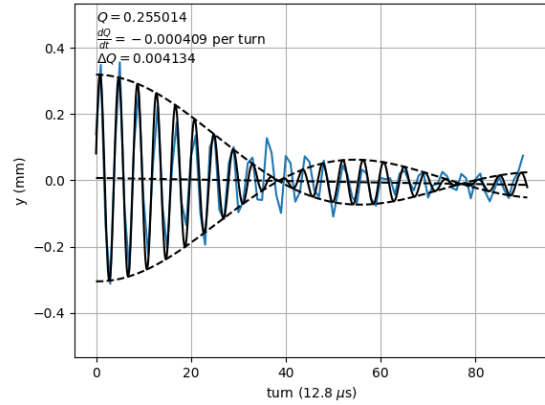
Figure 2: Fitting of the BPM data at top energy. The resulting tune, tune change per turn and tune spread are indicated. Due to the coupling between planes in this setting, the excitation of the beam in the horizontal plane after 30 turns can be seen in the vertical data.
