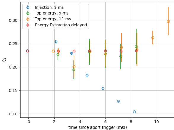
Figure 4: Reconstructed horizontal tunes during all four tests, the error bars come from the distribution of fitted tunes from the 160 BPMs.
