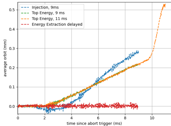
Figure 3: Average orbit offset around the RHIC ring as a function of time for all four tests.
