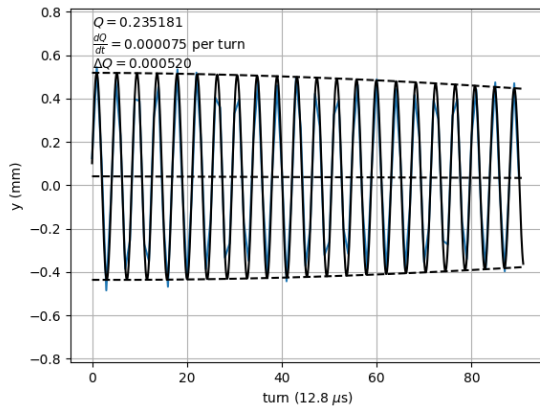
Figure 1: Fitting of the BPM data at injection energy. The resulting tune, tune change per turn and tune spread are indicated.
