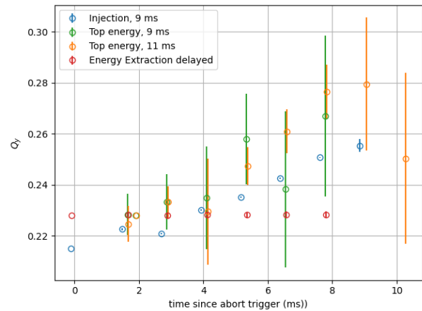
Figure 5: Reconstructed vertical tunes during all four tests, the error bars come from the distribution of fitted tunes from the 160 BPMs.
