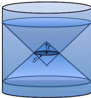
Figure 2: A small causal diamond in AdS consisting of the domain of dependence of the ball bounded by the holographic screen S . The ball lies in the t = 0 time slice, and is centered around the origin. The location of S with respect to the origin can be parametrized by the time t at which the inward future lightsheet arrives at the origin.
