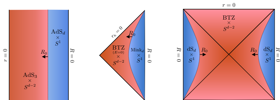
Figure 4: The first figure depicts, from left to right, the gluing of the [0, r_0] region of Weyl rescaled \text{AdS}_3 \times S^{d-2} to the [0, R_0] region of \text{AdS}_d \times S^1 . The second figure illustrates, from left to right, the gluing of the [0, r_0] region of massless (Weyl rescaled) \text{BTZ} \times S^{d-2} to the [0, R_0] region of \text{Mink}_d \times S^1 . Finally, the third figure shows the gluing of the [0, r_0] region of (Weyl rescaled) \text{BTZ} \times S^{d-2} to the [0, R_0] region of dS_d \times S^1 .
