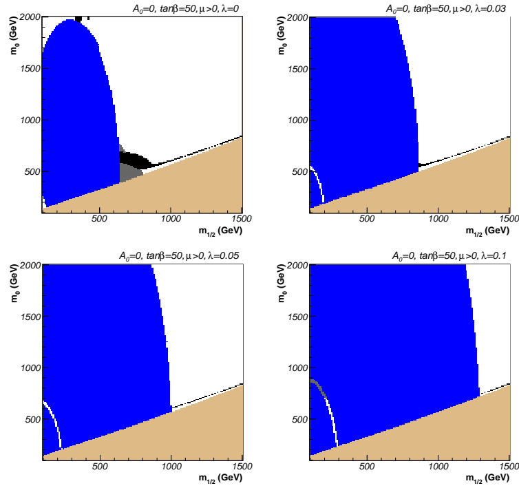
Figure 2.4: Same as Fig. 2.2 for \tan\beta = 50 , A_0 = 0 , \mu > 0 .
