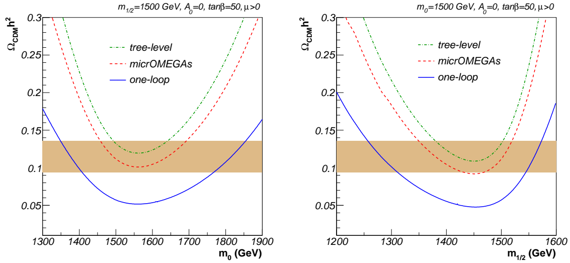
Figure 4.15: The prediction for the neutralino relic density \Omega_{\text{CDM}} h^2 as a function of the scalar mass parameter m_0 (left) and the gaugino mass parameter m_{1/2} (right) for our scenario 2 obtained with micrOMEGAs 2.1 including their cross section calculation (red dashed), our tree-level calculation (green dash-dotted), and our full one-loop QCD and SUSY-QCD cross section (blue solid) of the annihilation into b\bar{b} and t\bar{t} final states. The coloured band indicates the cosmologically favoured region at 2\sigma .
