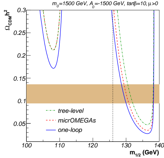
Figure 4.14: Prediction for the neutralino relic density \Omega_{\text{CDM}} h^2 as a function of the gaugino mass parameter m_{1/2} for our scenario 1. The coloured band indicates the cosmologically favoured region at 2\sigma , while the vertical dashed line separates the excluded (left) from the allowed (right) regions due to the LEP chargino-mass limit.
