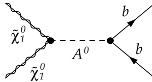
Figure 3.1: The leading order Feynman diagram of the neutralino annihilation process \tilde{\chi}\tilde{\chi} \rightarrow A^0 \rightarrow b\bar{b} .
