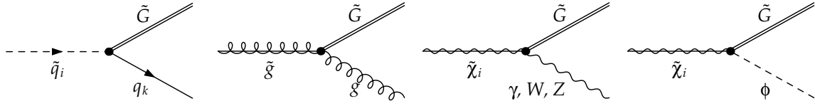
Figure 5.10: Leading order Feynman diagrams for the decay of a squark, a gluino, or a gaugino into its Standard Model partner and a gravitino.
