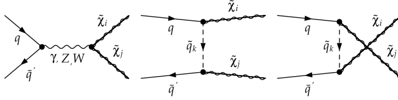
Figure 5.6: Tree-level Feynman diagrams for gaugino pair production.
