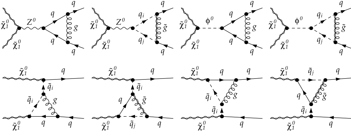
Figure 4.8: Vertex correction diagrams to the s -channel Z - and Higgs-boson exchange (top) and to the t -channel squark exchange (bottom) contributing at \mathcal{O}(\alpha_s) to the annihilation cross section. The corresponding u -channel squark-exchange diagrams are not shown.
