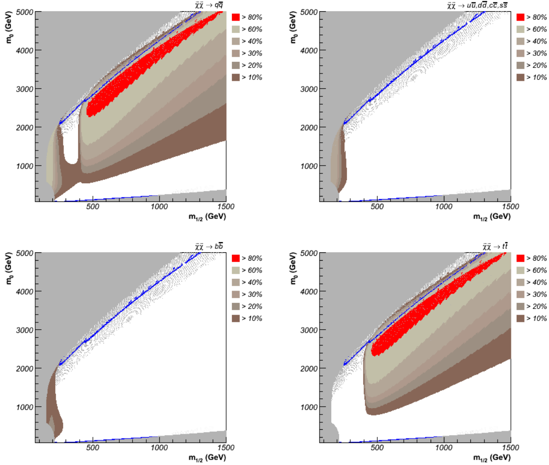
Figure 4.6: Same as Fig. 4.2 for \tan\beta = 10 and A_0 = 0 , where the SUSY mass spectrum has now been calculated with SuSpect 2.34. Grey shaded regions are excluded due to a charged LSP, no electroweak symmetry breaking, current LEP mass limits, or b \rightarrow s\gamma measurements.
