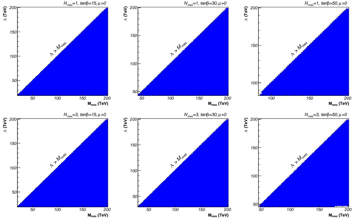
Figure 2.9: The \Lambda - M_{\text{mes}} planes for \tan \beta = 15, 30 , and 50 , N_{\text{mes}} = 1 and 3 , \mu > 0 . We show the b \rightarrow s\gamma excluded (dark blue) regions in constrained minimal flavour violation (cMFV). The region \Lambda > M_{\text{mes}} above the diagonal is theoretically excluded due to non-physical solutions to the renormalization group equations.
