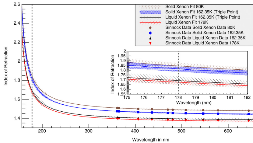
Fig. 3. Calculated index of refraction vs. wavelength (nm) for solid and liquid xenon. Source: The points show the data from Refs. [14] and [10].
