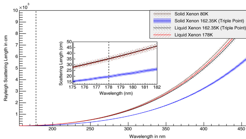
Fig. 4. Calculated Rayleigh scattering length (cm) vs. wavelength (nm) for solid and liquid xenon.
