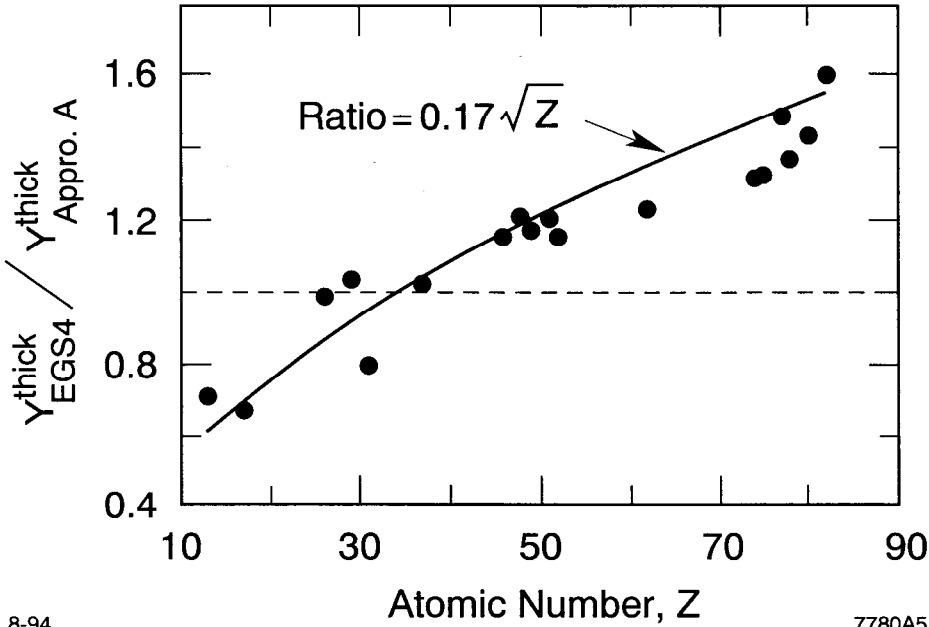
Figure 5. Ratio of the thick-target neutron yield calculated by EGS4 to that by Approximation A vs. the atomic number.
