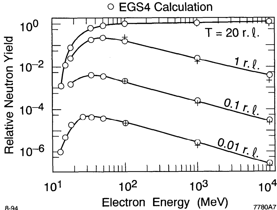
Figure 7. Relative neutron yields produced by bremsstrahlung in thick and thin iron targets as a function of the electron energy. The yield at 10 GeV and 20 r.l. is used as a normalizing point. The +-symbol shows the results of calculations using the scaling function (Eq. 15). The o-symbol shows the results of EGS4 calculations with a solid line drawn through them.
