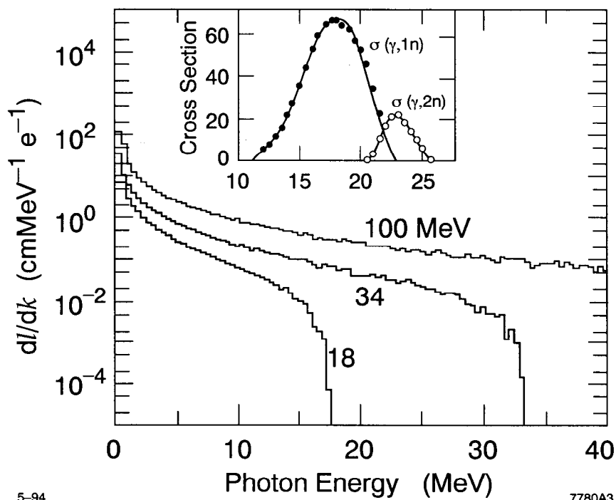
Figure 3. Differential photon track length distributions produced in thick iron targets struck by 18 MeV, 34 MeV, and 100 MeV electrons.
