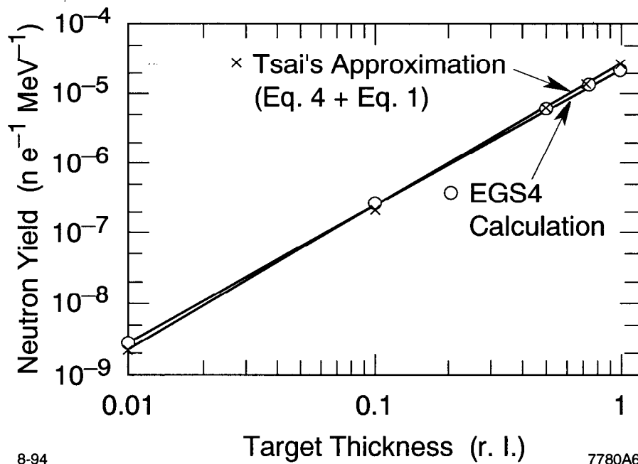
Figure 6. Neutron yields produced by bremsstrahlung in thin iron targets struck by 100 MeV electrons as a function of the target thickness.
