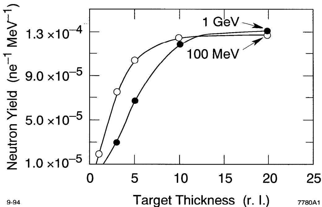
Figure 1. Neutron yield as a function of iron-target thickness for 100 MeV and 1 GeV electron beams.
