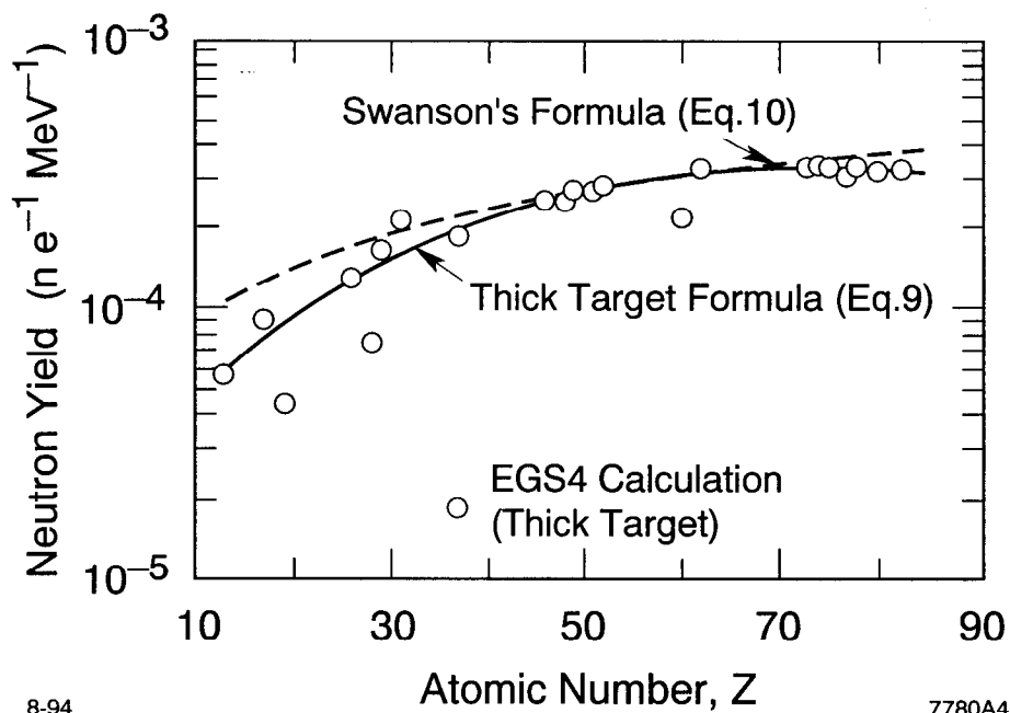
Figure 4. Neutron yields produced in thick targets struck by 100 MeV electrons as a function of the atomic number.
