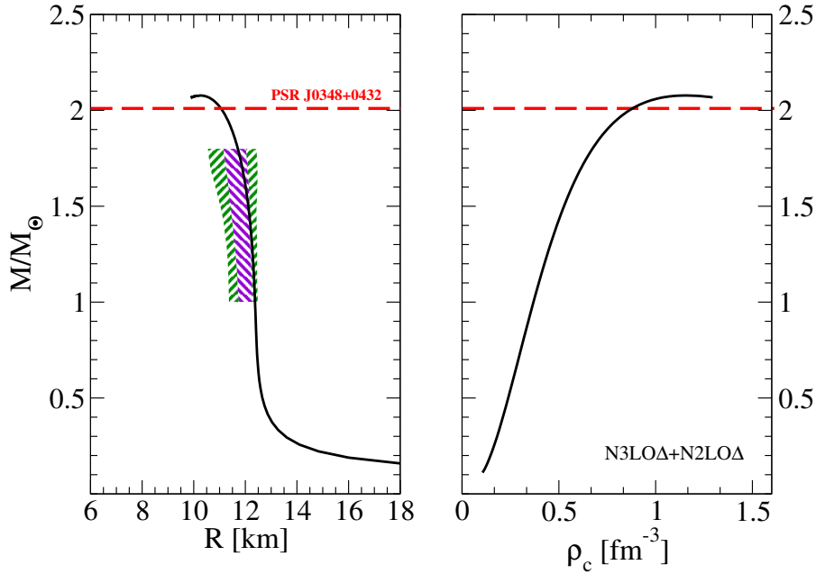
Figure 2. Mass-radius relationship (left panel) and mass-central density relationship (right panel) for the N3LOΔ+N2LOΔ model. The hatched region in the left panel represents the mass-radius constraints obtained in [52, 53]. The red dashed line stands for the measured mass of PSR J0348+0432 [30]. M_{\odot} = 1.9885 \times 10^{33} g is the mass of the sun.
