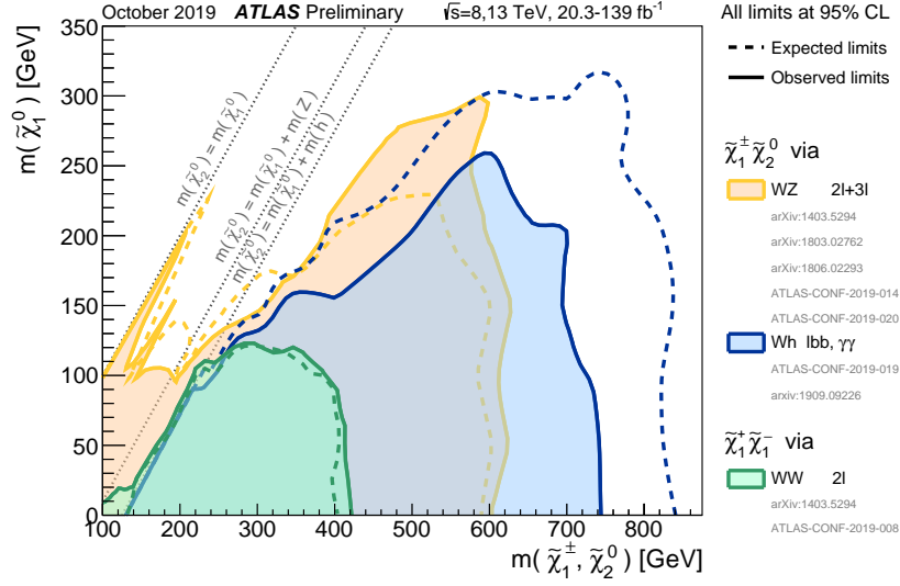
Figure 14: The 95% CL exclusion limits on \tilde{\chi}_1^+ \tilde{\chi}_1^- and \tilde{\chi}_1^\pm \tilde{\chi}_2^0 production with SM-boson-mediated decays, as a function of the \tilde{\chi}_1^\pm , \tilde{\chi}_2^0 and \tilde{\chi}_1^0 masses. The production cross-section is for pure wino \tilde{\chi}_1^+ \tilde{\chi}_1^- and \tilde{\chi}_1^\pm \tilde{\chi}_2^0 . Each individual exclusion contour represents a union of the excluded regions of one or more analyses.
