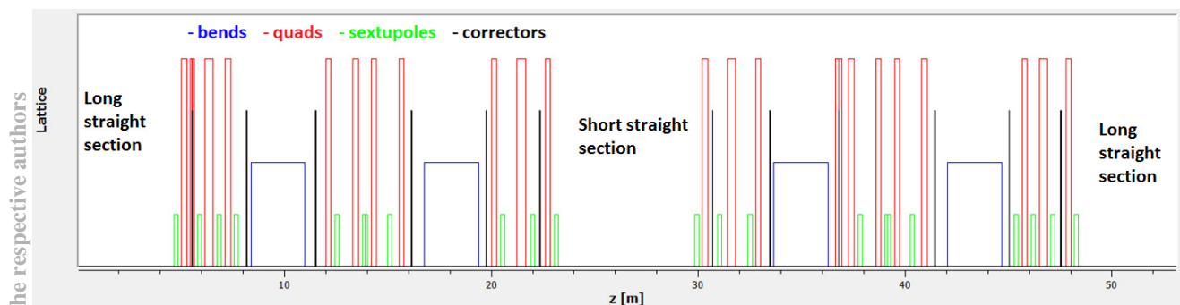
Figure 1: NSLS-II SR lattice.
