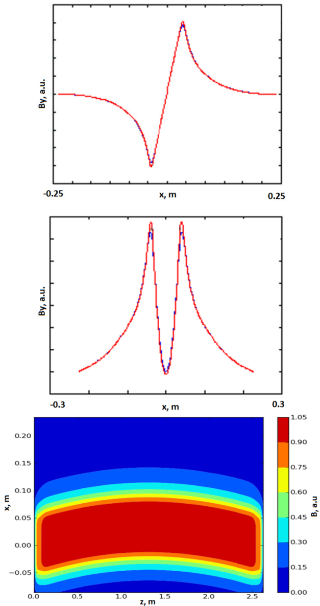
Figure 2: Profiles of magnetic field for quadrupole (top), sextupole (middle) and dipole (bottom) in the SR.
