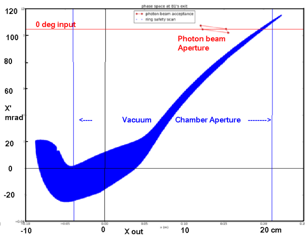
Figure 5: Beam particle phase space (blue dots) at the exit of the first dipole. Also shown are the photon beam aperture around the input beam direction and the dipole vacuum chamber apertures.
