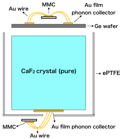
Figure 3. A schematic view of a \text{CaF}_2 scintillating bolometer for heat and light detection. A \text{CaF}_2 (pure) of 5cm diameter and 5cm height was used as the absorber crystal. A 2 cm diameter gold film on the \text{CaF}_2 surface transfers the heat to an MMC phonon sensor via gold wires. This heat channel measures the major energy deposit to the crystal. Scintillation photons absorbed in the 2 inch Ge wafer are measured with another MMC photon sensor.
