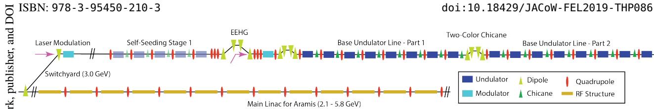
Figure 1: Layout of the Athos beamline.
