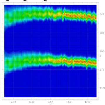
Figure 10: Longitudinal phase distribution of the bunch over the boosting time.
