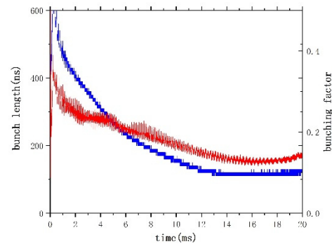
Figure 7: Bunch length (blue) and bunching factor (red).
