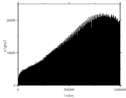
Figure 5: wall current with DC part subtracted. For convenience in data analysing, a factor -1 is multiplied to the signal.
