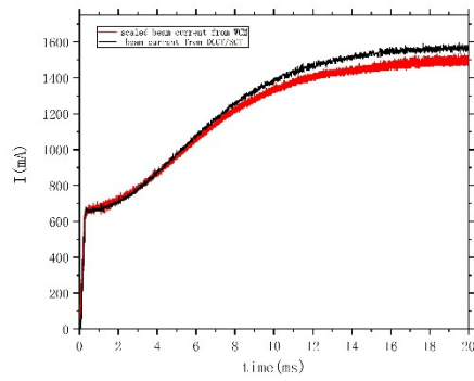
Figure 4: Peaks of the positive part of the wall current data (red) vs. beam current from DCCT/SCT (black).
