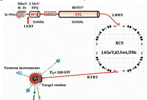
Figure 1: Layout of China Spallation of neutron Source.
