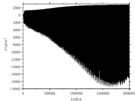
Figure 2: Real wall current data extracted from WCM.
