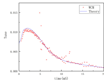
Figure 8: Tune measured from WCM and theoretical calculation.
