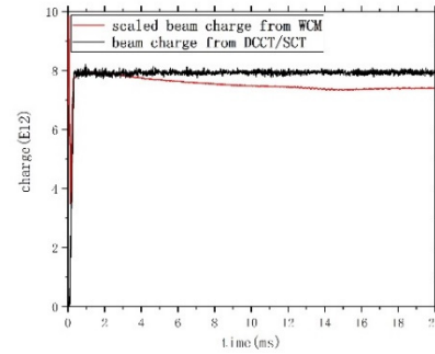
Figure 6: proton charge derived from WCM (red) vs. proton charge from DCCT/SCT over boosting time.
