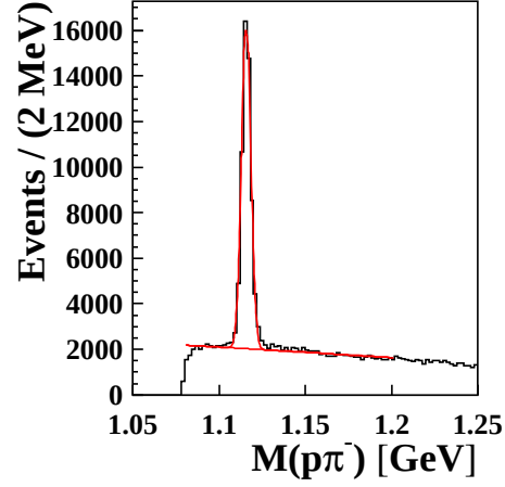
Fig.2. Invariant mass distribution of the p\pi^- and charge conjugate (c.c.) system.
