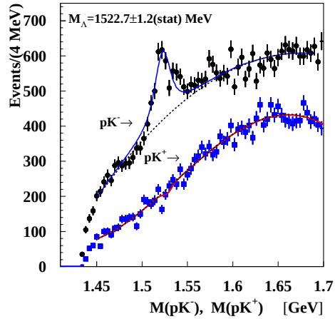
Fig.4. Spectra of the invariant mass distributions M_{pK^-} (top) and M_{pK^+} (bottom). A clear peak is seen for the \Lambda(1520) in the M_{pK^-} invariant mass distribution, but none for the hypothetical \Theta^{++} peak near 1530 MeV.
