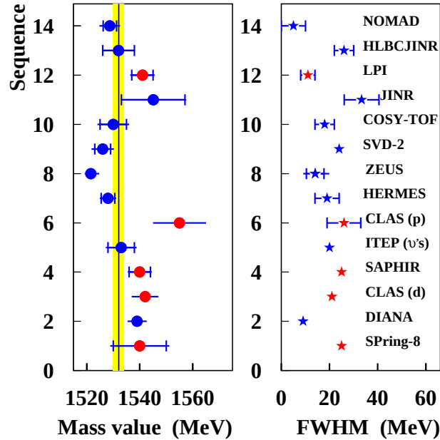
Fig. 10. Mass values and experimental FWHM widths observed in various experiments search for the hypothetical \Theta^+ state, as of January 2005. The hatched area corresponds to the weighted average (1532.1 \pm 2.1) of all data \pm 1 standard deviation. The uncertainty of the average was scaled by the usual factor of square root of the reduced \chi^2 .
