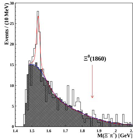
Fig. 6. Invariant mass distribution of the p\pi^-\pi^-\pi^+ (plus c.c.) system, subject to the constraints on the event topology discussed in the text. The arrow shows the hypothetical \Xi_{3/2}^0 mass. The excess near 1770 MeV has a statistical significance of only 1.8\sigma . The peak near 1530 MeV represents the \Xi^0(1530) resonance.
