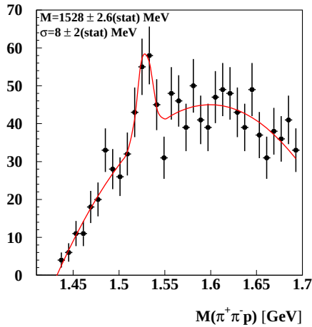
Fig. 7. Distribution in invariant mass of the p\pi^+\pi^- system. The smooth curve results from a fit to the data of a Gaussian plus a third-order polynomial.
