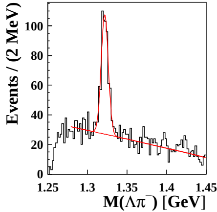
Fig.3. Invariant mass distribution of the p\pi^-\pi^- plus (c.c.) system. The peak near 1.32 GeV corresponds to the excitation of the \Xi^-(1321) resonance.
