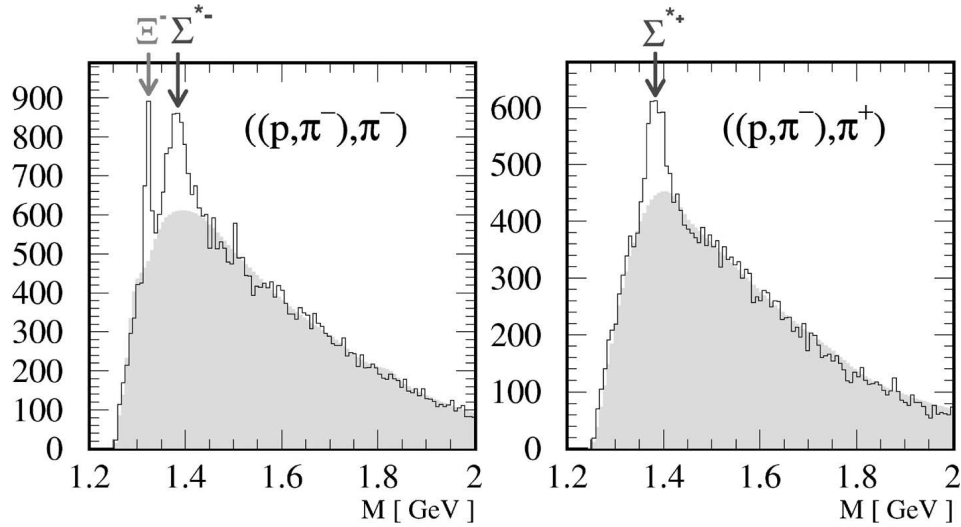
Fig. 9. Distribution in invariant mass of the (p\pi^-)\pi^- (left panel) and (p\pi^-)\pi^+ (right panel) system. The mixed event spectrum is shown as a shaded histogram [40].
