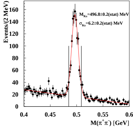
Fig.1. Invariant M_{\pi^+\pi^-} distribution. A window corresponding to \pm 2\sigma is shown by the vertical lines.
