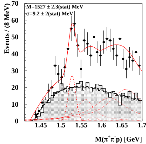
Fig. 8. The same as in Fig. 7, but with a different description of the background (see description in text).
