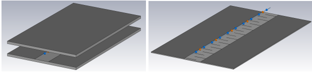
Figure 2: Left: Simplified parallel plate model of the HTS-SCU for resistive wake simulations. Right: Model of the laser-scribed HTS tape on top of the stainless steel core.
