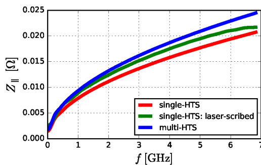
Figure 4: Longitudinal resistive wall impedance with and without laser-scribed sections and for a multi-layered HTS.
