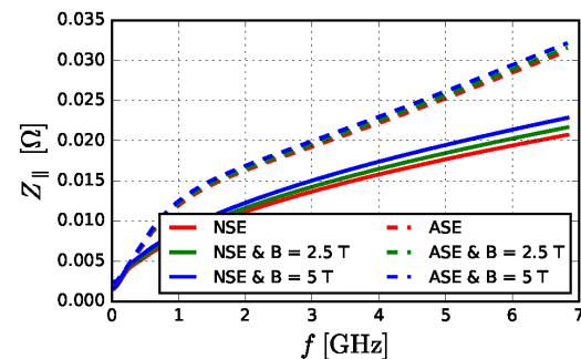
Figure 5: Longitudinal resistive wall impedance including ASE and magnetoresistance. NSE stands for normal skin effect.
