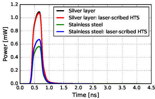
Figure 6: Resistive loss power in the silver layer and stainless steel for a single bunch excitation.
