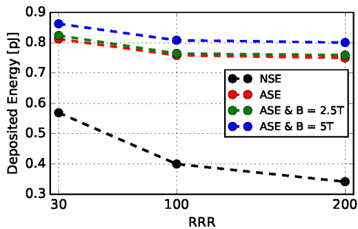
Figure 7: Total deposited thermal energy for a single bunch as a function of RRR taking into account the ASE and magnetoresistance.
