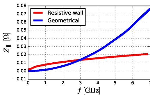
Figure 3: Longitudinal geometrical and resistive wall impedance computed with the models in Figs. 1 and 2, respectively. In the simulations, a smooth silver layer with nominal conductivity is considered.
