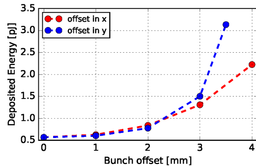
Figure 9: Total deposited energy in the case of a bunch offset.
