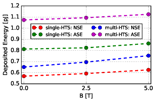
Figure 8: Thermal energy deposited by a single bunch as a function of the external magnetic field in the case of single and multiple HTS tapes.
