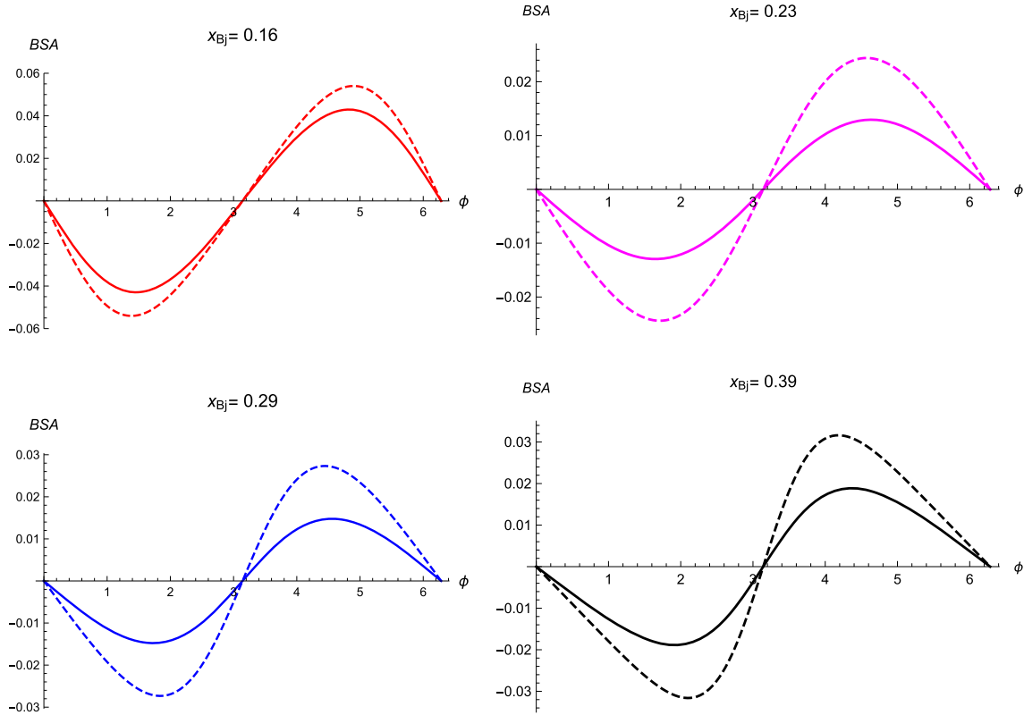
Fig. 3 Beam-spin asymmetry (BSA) for four values of x_{\text{Bj}} , the solid line is for \theta_C = \pi/36 , the dashed line for \theta_C = \pi/18
