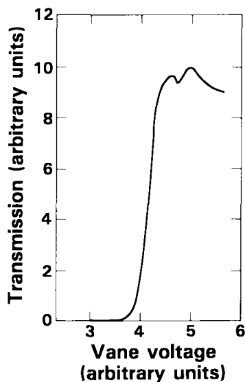
Fig. 2: Transmission of fully accelerated \text{N}^{+3} beam as a function of vane voltage.
