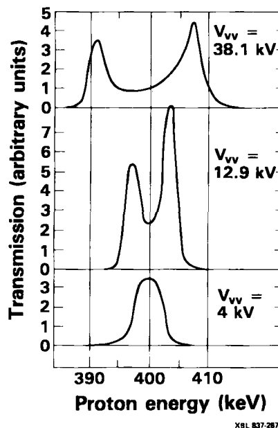
Fig. 5: Output energy spectra of the drift-through 400 keV proton beam for three different values of the vane-vane voltage V_{vv} .
