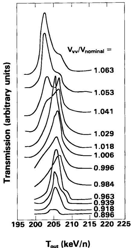
Fig. 4: \text{N}^{+3} energy spectra for several values of the vane-vane voltage V_{vv} .
