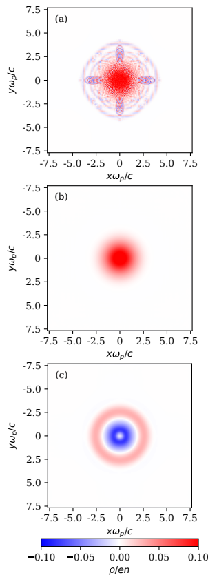
Figure 4: Transverse distributions of the plasma charge density: (a) the conventional solver, \xi = -1000c/\omega_p , (b) the improved solver, \xi = -1000c/\omega_p , and (c) the improved solver, \xi = -2300c/\omega_p .
