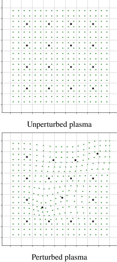
Figure 1: Schematic arrangement of “real” (black stars) and “virtual” (green dots) macro-particles using the dual plasma approach.
