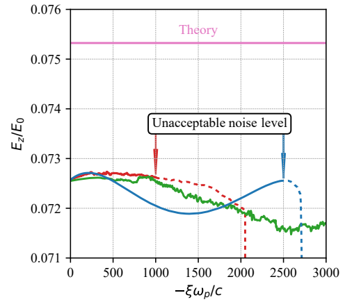
Figure 2: Positive local extrema of the on-axis electric field E_z in test 1 calculated with LCODE (green line), LCODE3D with conventional (red line) and improved (blue line) solvers.
