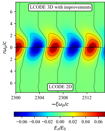
Figure 3: Comparison of field profiles after a long-term wave evolution.
