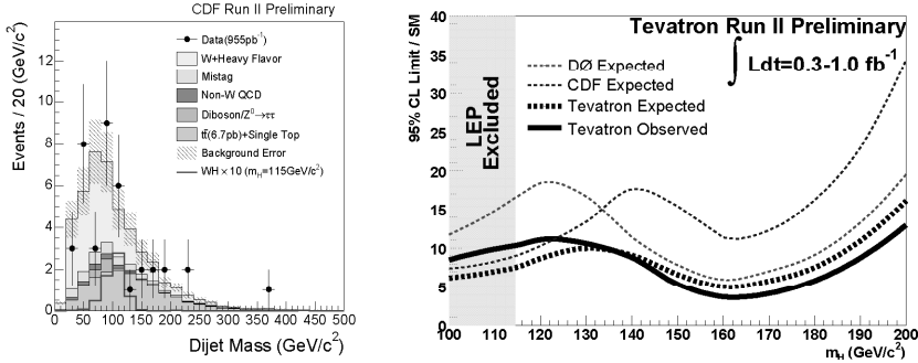
Figure 1: Left: dijet mass distribution in W + \geq 2 jets events with two secondary vertex tags. Right: combined CDF and DO limits on SM Higgs production, normalized to the predicted SM cross section.
