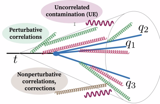
Figure 5.1: Sketch of the different sources of radiation entering in the catchment area of a top-initiated large- R jet.
