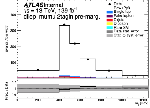
(b) m_{t\bar{t}} , \mu\mu channel, 2- b incl.
