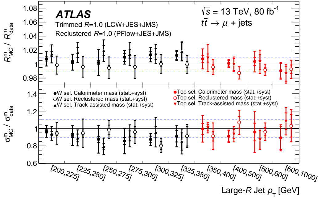
Figure 4.11: The relative Jet Mass Scale and Resolution for several jet mass definitions as a function of the jet p_T . Black and red markers represent results for W -like and top-like jets. The inner error bar stands for the statistical uncertainty and the outer error bar includes the statistical and systematic uncertainty. Dashed blue lines, corresponding to \pm 1\% for the JMS and \pm 10\% for the JMR, are drawn for reference. Figure taken from Ref. [197].
