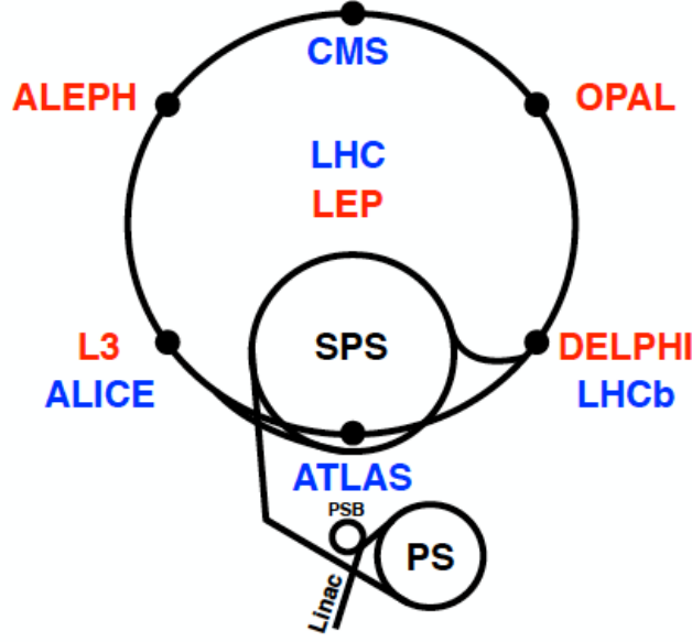
Figure 3.1: Sketch of the CERN accelerator complex with the experimental detectors placed at each interaction point in the LHC (blue) and LEP (red) era.
