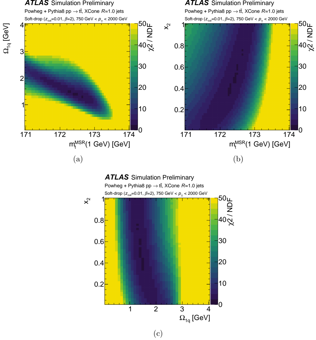
Figure 5.17: The \chi^2 results as a function of the MSR mass m_t^{\text{MSR}}(1 \text{ GeV}) and the parameters of the shape function \Omega_{1q}^{\circ\circ} and x_2 , obtained from the fit with the NLL prediction of Ref. [210] to the particle-level jet mass distribution for boosted top quarks in the nominal ATLAS POWHEG +PYTHIA 8 sample. The results are shown in the two-dimensional plane of (a) MSR mass versus \Omega_{1q}^{\circ\circ} , (b) MSR mass versus x_2 and (c) \Omega_{1q}^{\circ\circ} versus x_2 . In each case, the 2D distribution is obtained by marginalizing over the third parameter. The three parameters of the calculation are varied to find the best description of the three p_T intervals used in the calibration procedure.
