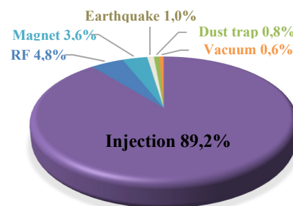
Figure 3: Breakdown of the failure time in FY 2020 for PF-AR.
