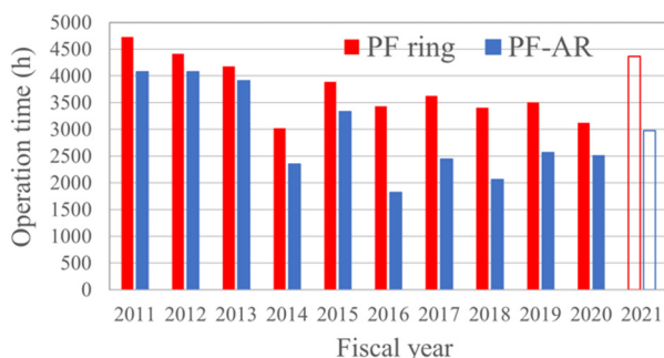
Figure 1: Operation times of PF-ring and PF-AR over ten years.
