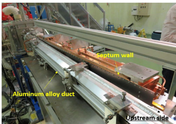
Figure 4: Reconstruction work of a septum magnet and beam ducts of the injection section of PF-ring.
