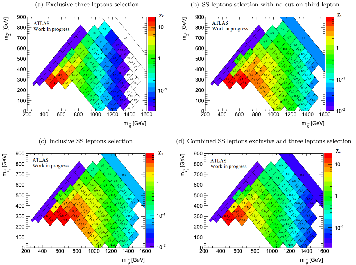
Figure 7.2: Example of sensitivity gain in \tilde{g}\tilde{g} production in 2-step decay simplified model after combining the SS and 3 leptons analyses ( \sqrt{s} = 8 TeV, L = 20.3 fb ^{-1} ). On the z axis the real or combined significance is shown.
