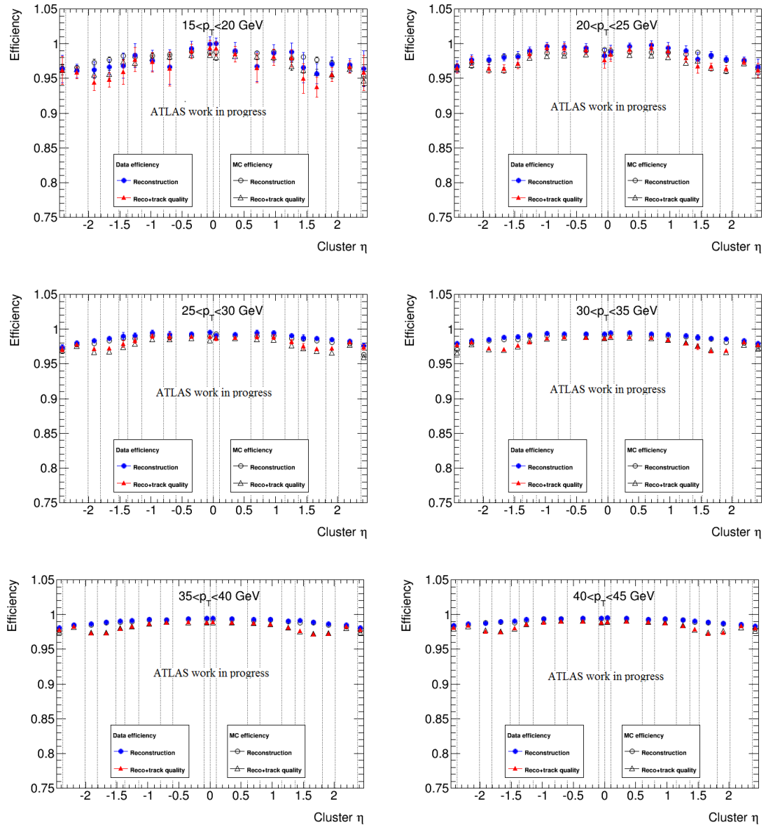
Figure A.3: Electron reconstruction and reconstruction + track quality efficiencies in data (filled markers) and MC (empty markers) in several (\eta, p_T) bins. \sqrt{s} = 8 TeV and L = 20.3 \text{ fb}^{-1} . Only combined statistical and systematic uncertainties are shown.
