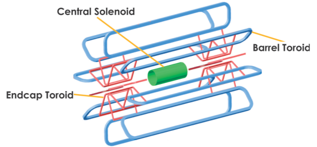
Figure 3.12: Magnet system [152].
