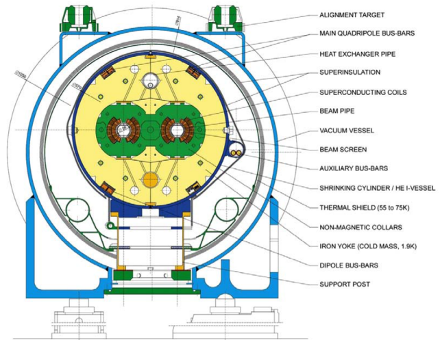
Figure 3.2: Cross section of the LHC dipole [145].
