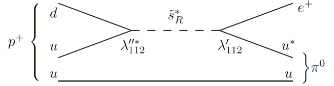
Figure 2.2: Illustrative Feynman diagram for the proton decay.
