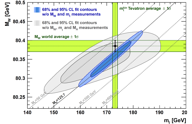
Figure 1.2: Contour plots showing the consistency between several direct and indirect Standard Model physical observables measurements [62].
