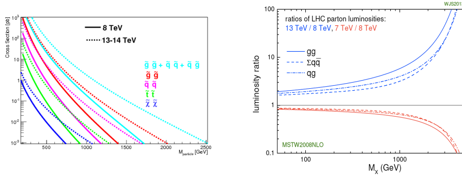
Figure 8.4: Left plot : SUSY particles production cross section at 8 TeV (bold line) and 13 TeV [294]. Right plot : Ratios of LHC parton luminosities [295].
