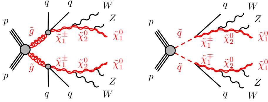
Figure 7.1: Feynman diagrams representative for the gluino mediated and direct production of 1 st and 2 nd generation squarks decaying to WZWZ model.
