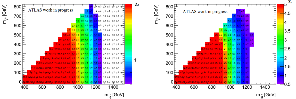
Figure 7.7: Considering the gluino mediated virtual top squark \tilde{g} \rightarrow t\bar{t}\tilde{\chi}_1^0 model, the signal regions combination giving the best significance in each point (left) and the significance obtained with the signal regions combination corresponding to index 3 (right) are shown. On the z axis the combined significance, Z_c is showed ( \sqrt{s} = 8 TeV, L = 20.3 fb ^{-1} ).
