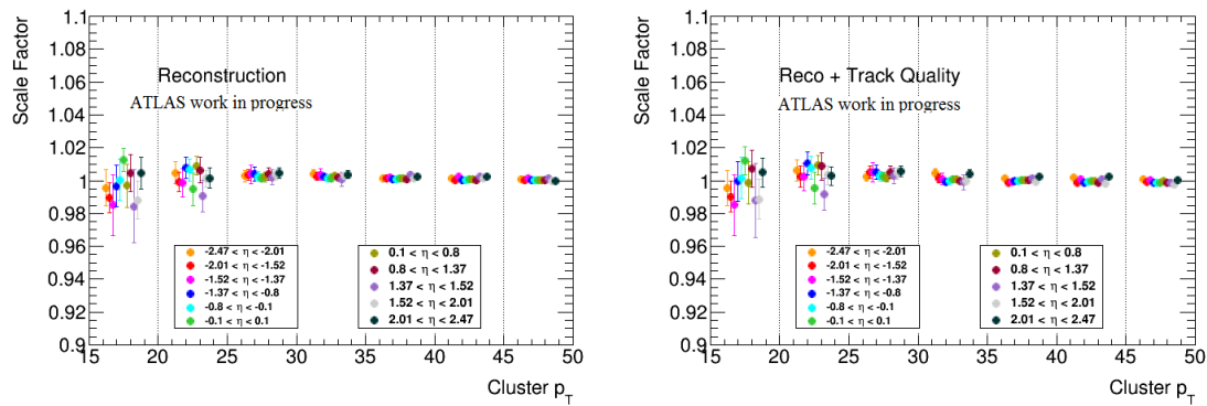
Figure A.4: Electron scale factors at reconstruction (left) and reconstruction + track quality (right) stages. \sqrt{s} = 8 TeV and L = 20.3 \text{ fb}^{-1} . Only the total uncertainty is considered.
