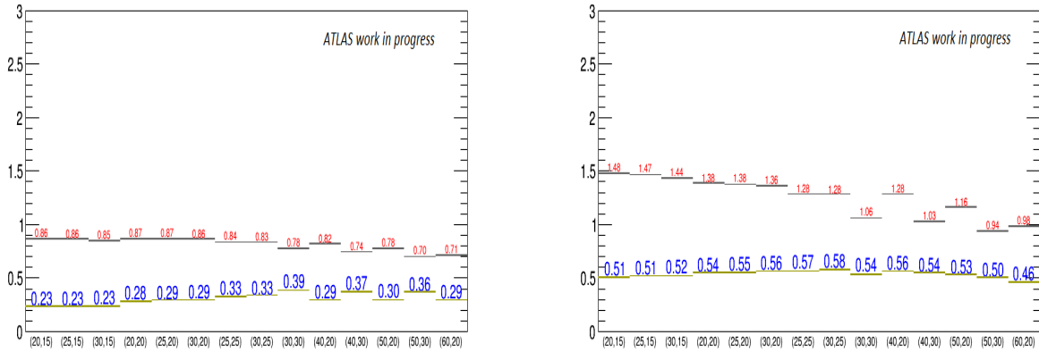
Figure 9.9: Optimization of the lepton p_T threshold cuts in SR1b (left) and SR2b (right). Numbers for the Z_r ( Z_0 ) significance shown in bold blue (red) are obtained at 14 TeV for 20 \text{fb}^{-1} of data.
