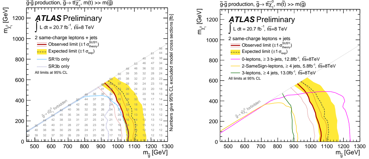
Figure 6.19: Expected and observed limits for gluino pair production via a virtual top squark, \tilde{g} \rightarrow t\bar{t}\tilde{\chi}_1^0 model. The importance of each signal region is shown in the left plot. A comparison with all ATLAS analyses available at the time of publication is shown on the right side plot. With dark orange are shown the results of the of this search using 5.8 \text{ fb}^{-1} of 8 TeV data.
