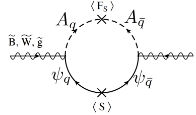
Figure 2.5: Illustration of the messenger - gauginos coupling.
