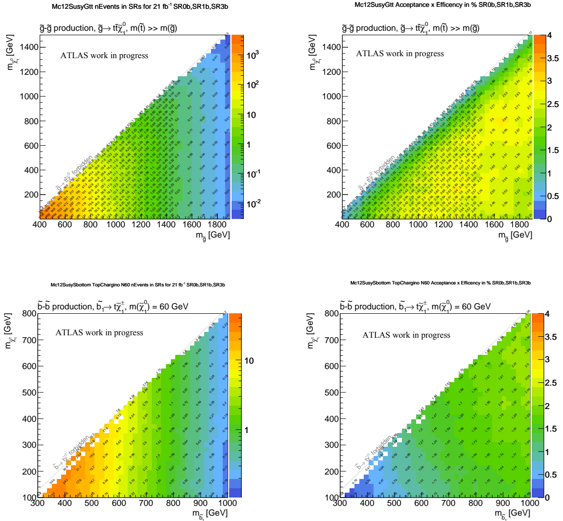
Figure 6.5: Number of signal events passing the combined SRs cuts (left) together with the A \times \epsilon (right) in two models: gluino pair production via virtual top squark (top) and direct bottom squarks production (bottom).
