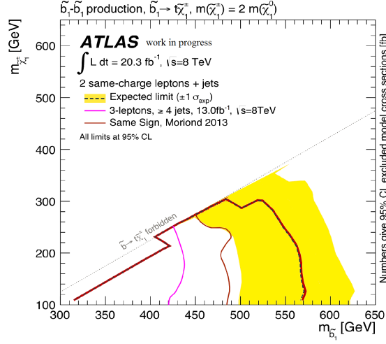
Figure 7.9: Expected exclusion limit for direct bottom squark production model after the signal regions re-optimization ( \sqrt{s} = 8 TeV, L = 20.3 \text{ fb}^{-1} ). Previous limits (Moriond 2013) are shown with dark orange line.
