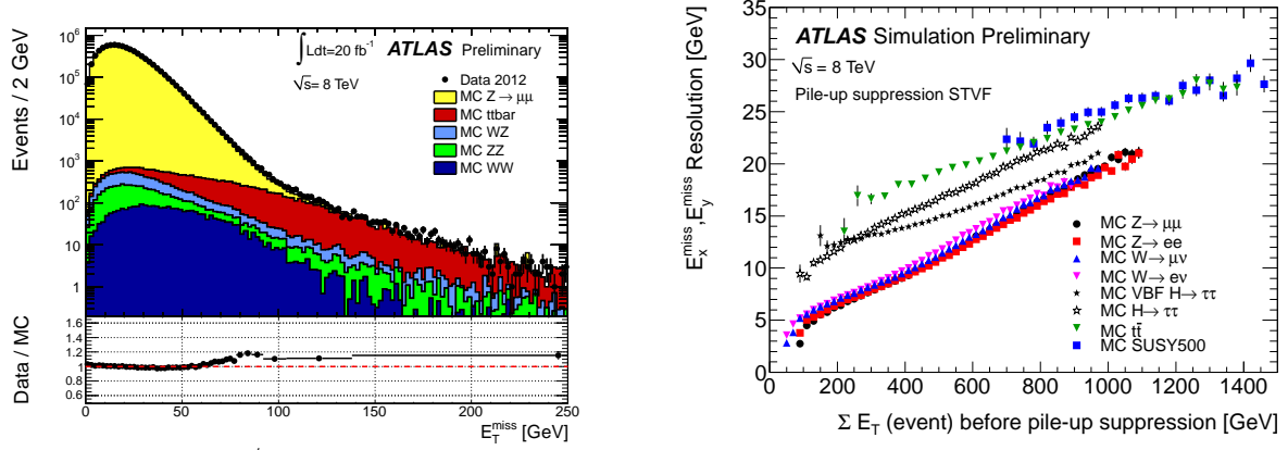
Figure 4.14: Left : E_T distribution as measured in data with Z \rightarrow \mu\mu events without pile-up suppression [211]. Right : E_T resolution summary plot [211].
