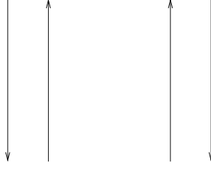
Figure 2.9: Pairs of paths that are positively and negatively oriented, respectively.
