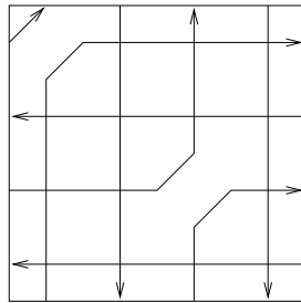
Figure 2.7: Left: An incorrect way of making two (1,1) paths. They intersect each other, which implies that the adjacent nodes are not properly ordered. Right: The correct way of making two (1,1) paths.
