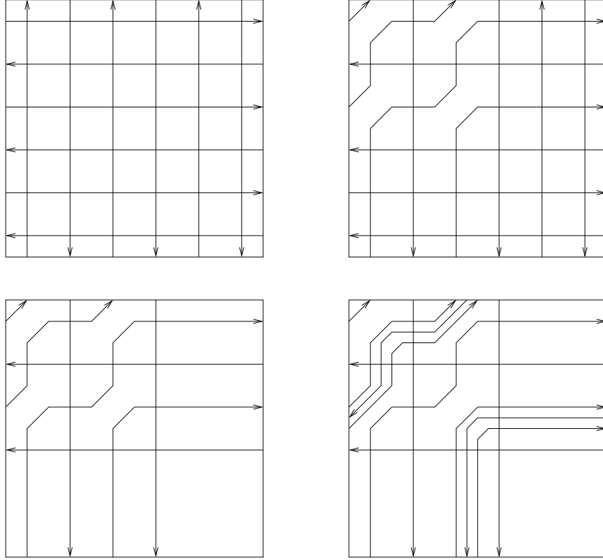
Figure 2.12: Creating three (1,1) paths and one (-1,1) path without introducing extra crossings. We first make two (1,1) paths and then add a (1,1) - (-1,-1) pair that follows one of those two paths.
