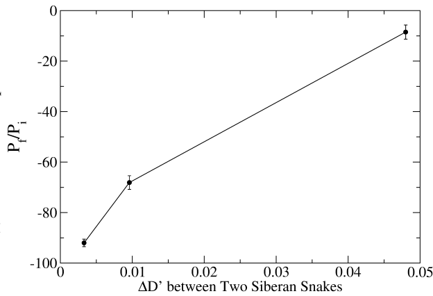
Figure 2: The average final to initial polarization ratio for 3 sec sweep time at injection as function of \Delta D' at the two Siberian Snakes. The small \Delta D' is critical for full spin flip.
