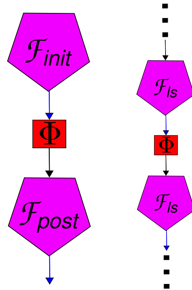
Fig. 4 Left: Traditional QAA or reverse annealing initialised based on the outcome of a classical algorithm formulated in terms of inference primitives and processing functions, where \mathcal{F}_{\text{init}} is defined in Eq. (11). Right: local search protocol formulated in terms of inference primitives and processing functions, the general for \mathcal{F}_{\text{ls}} is given in Eq. (12)
