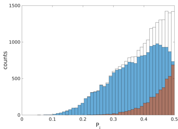
Fig. 2 Histogram of P_i for spin values obtained by the ‘traditional’ QAA on 1500 instances of spin glass problems described by Eq. (6) with n = 17 , ( 1500 \times (n - 1) = 24,000 data points). Data are based on PIQA runs with T = 0.8246 and \tau = 20 using the same numerical methods as the proof of principle in Chancellor (2017). Blue (light gray in print) bars are cases where S_i found by Eq. (7) agrees with the true ground state, red (dark gray in print) are cases where it does not, and unfilled bars are total counts
