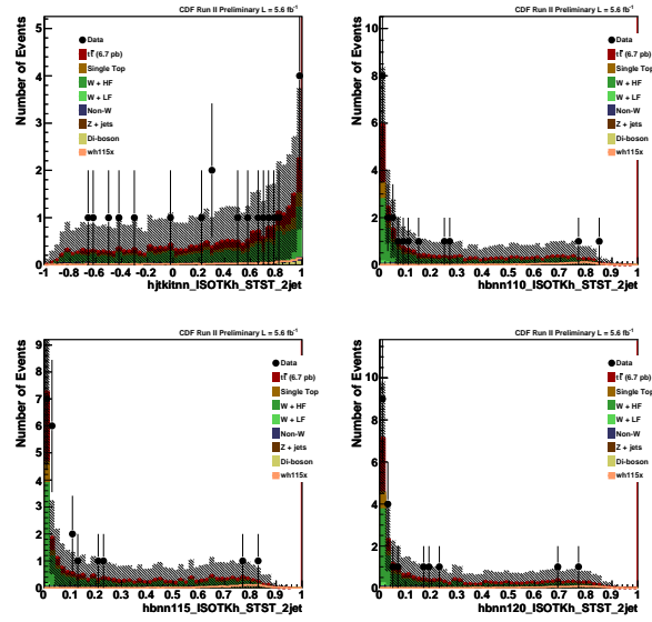
Figure 22: STST kinematic distributions for kitnn and Bnn output corresponds to m_H = 110, 115, 120 \text{ GeV}/c^2 respectively.
