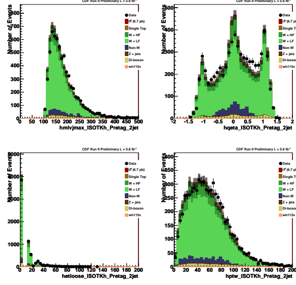
Figure 15: Pretag kinematic distributions for maximum of lv_j mass, \eta \times Q , sum loose jet E_T , and P_T of W candidate.
