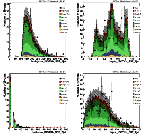
Figure 36: SST kinematic distributions for maximum of lv_j mass, \eta \times Q , sum loose jet E_T , and P_T of W candidate.
