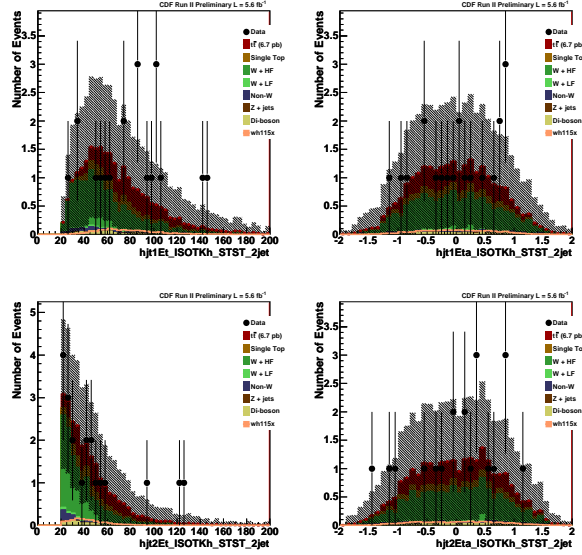
Figure 19: STST kinematic distributions for first jet E_T , \eta and second jet E_T , \eta .
