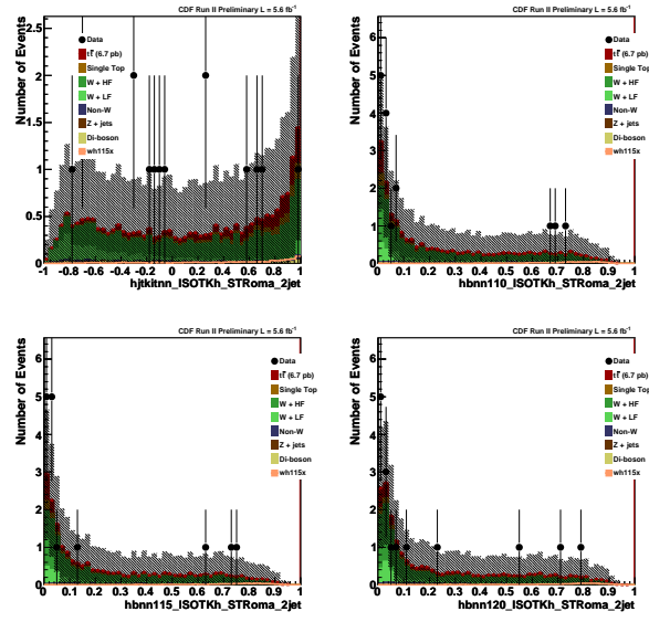
Figure 32: STRoma kinematic distributions for kitnn and Bnn output corresponds to m_H = 110, 115, 120 \text{ GeV}/c^2 respectively.
