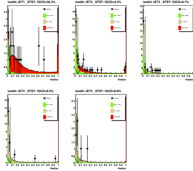
Figure 5: QCD fraction estimate for ST+ST of the W + \text{jets} events.
