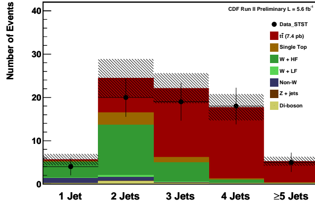
Figure 9: Number of expected and observed events for ST+ST tag category.
