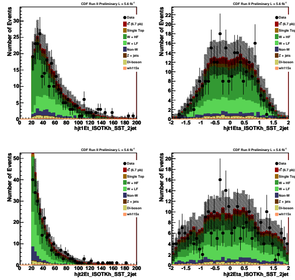
Figure 34: SST kinematic distributions for first jet E_T , \eta and second jet E_T , \eta .
