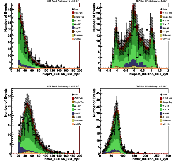
Figure 33: SST kinematic distributions for isolated track p_T , \eta , E_T , and W transverse mass.
