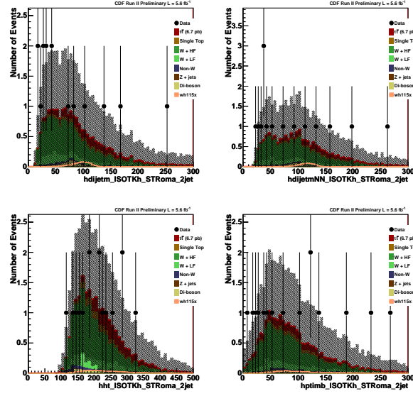
Figure 30: STRoma kinematic distributions for dijet mass before and after bjet energy correction, H_T , and P_T imbalance.
