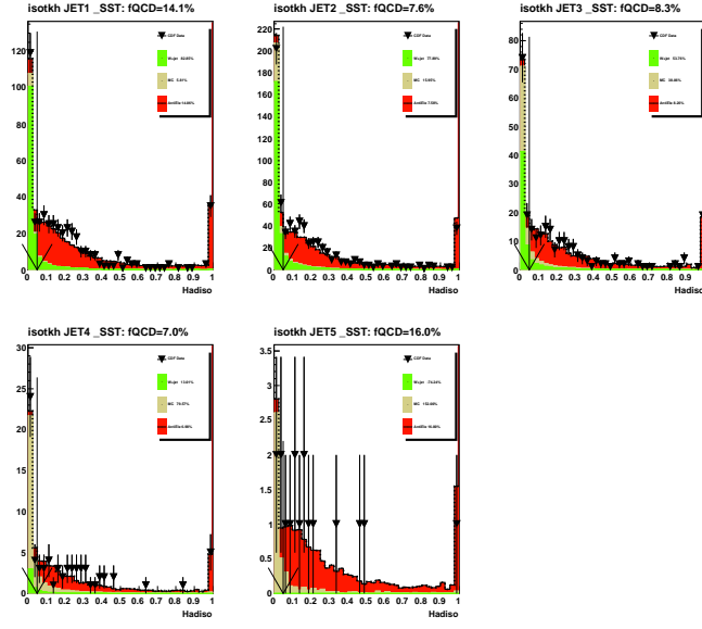
Figure 4: QCD fraction estimate for 1-ST of the W + \text{jets} events.
