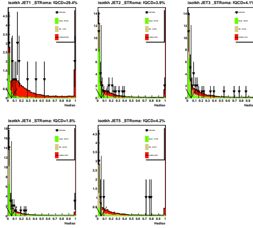
Figure 7: QCD fraction estimate for ST+RomaNN of the W + jets events.
