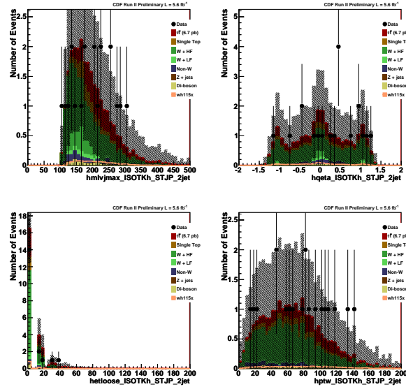
Figure 26: STJP kinematic distributions for maximum of lv_j mass, \eta \times Q , sum loose jet E_T , and P_T of W candidate.
