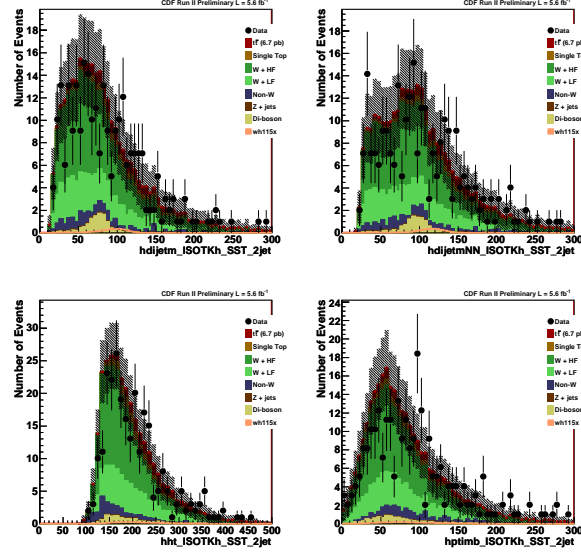
Figure 35: SST kinematic distributions for dijet mass before and after bjet energy correction, H_T , and P_T imbalance.
