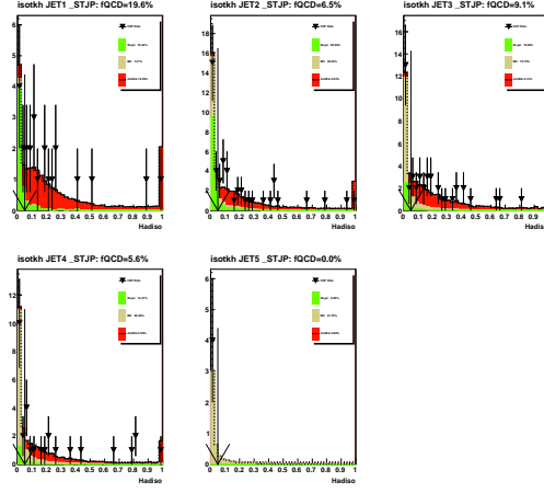
Figure 6: QCD fraction estimate for ST+JP of the W + jets events.
