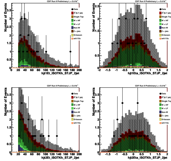
Figure 24: STJP kinematic distributions for first jet E_T , \eta and second jet E_T , \eta .
