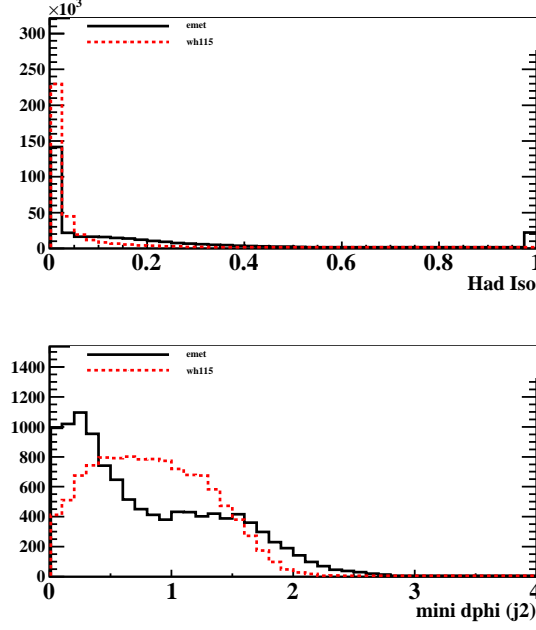
Figure 1: Comparison of the hadronic isolation and the minimum \Delta\phi between E_T and jets for isolated track candidates from the E_T trigger data and the WH115 MC.
