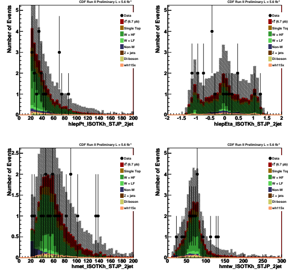
Figure 23: STJP kinematic distributions for isolated track p_T , \eta , E_T , and W transverse mass.
