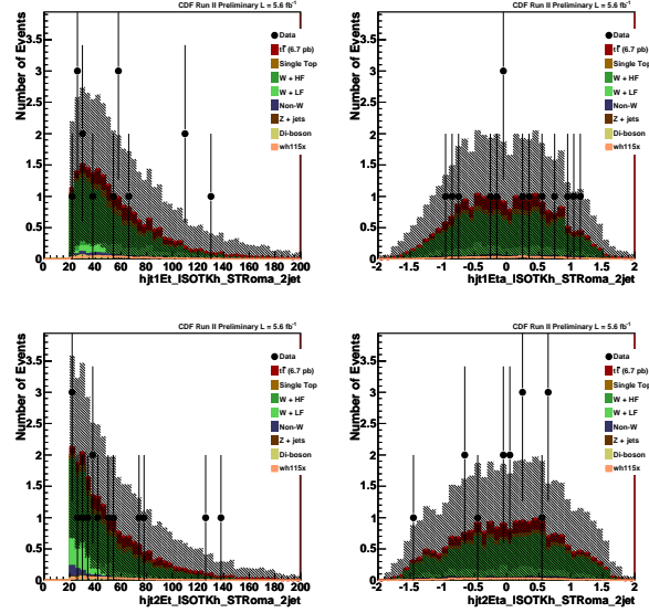
Figure 29: STRoma kinematic distributions for first jet E_T , \eta and second jet E_T , \eta .
