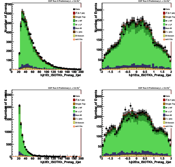
Figure 13: Pretag kinematic distributions for first jet E_T , \eta and second jet E_T , \eta .
