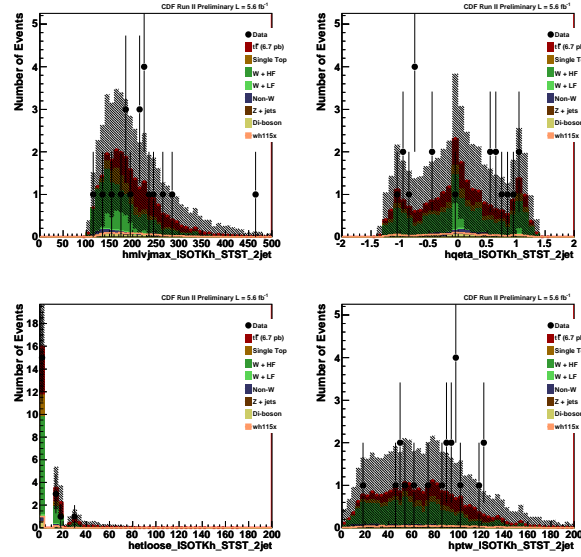
Figure 21: STST kinematic distributions for maximum of lvj mass, \eta \times Q , sum loose jet E_T , and P_T of W candidate.
