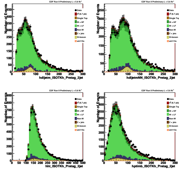
Figure 14: Pretag kinematic distributions for dijet mass before and after bjet energy correction, H_T , and P_T imbalance.
