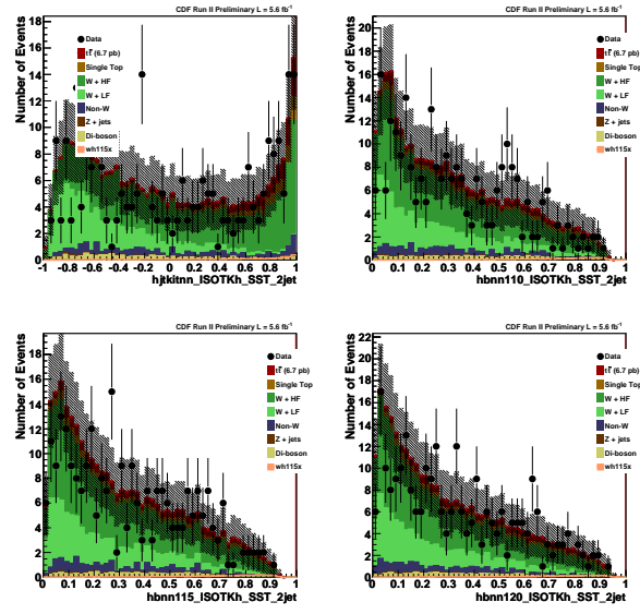
Figure 37: SST kinematic distributions for kitnn and Bnn output corresponds to m_H = 110, 115, 120 GeV/c 2 respectively.
