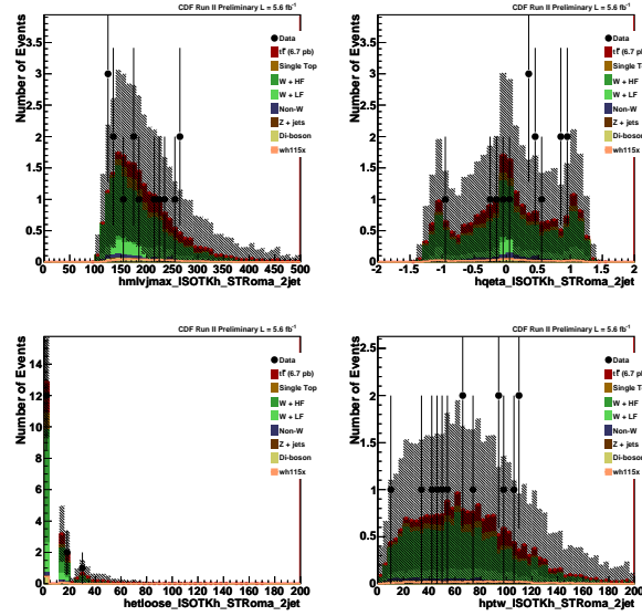
Figure 31: STRoma kinematic distributions for maximum of lvj mass, \eta \times Q , sum loose jet E_T , and P_T of W candidate.
