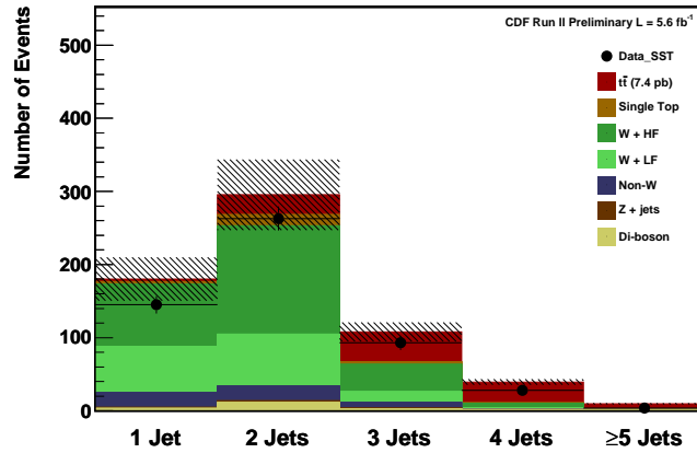
Figure 8: Number of expected and observed events for 1-ST tag category.
