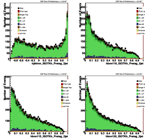
Figure 16: Pretag kinematic distributions for kitnn and Bnn output corresponds to m_H = 110, 115, 120 \text{GeV}/c^2 respectively.
