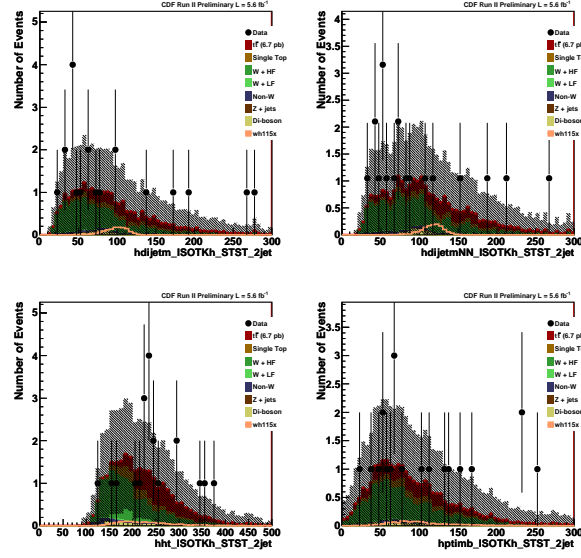
Figure 20: STST kinematic distributions for dijet mass before and after bjet energy correction, H_T , and P_T imbalance.
