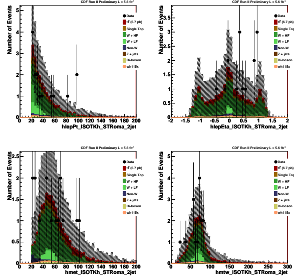
Figure 28: STRoma kinematic distributions for isolated track p_T , \eta , E_T , and W transverse mass.
