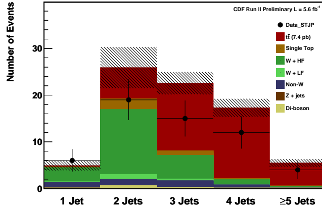
Figure 10: Number of expected and observed events for ST+JP tag category.
