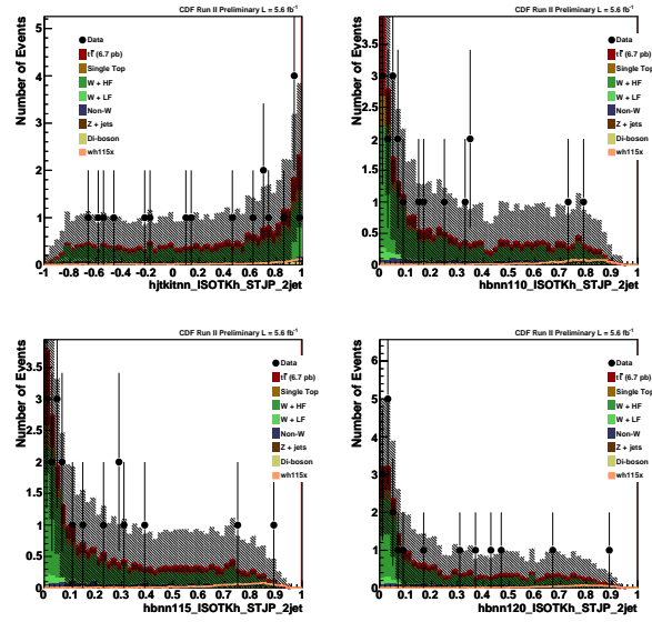
Figure 27: STJP kinematic distributions for kitnn and Bnn output corresponds to m_H = 110, 115, 120 \text{ GeV}/c^2 respectively.
