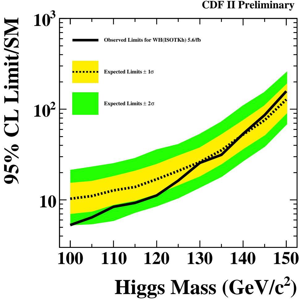
Figure 17: Expected and observed limits for combining all b -tag categories.
