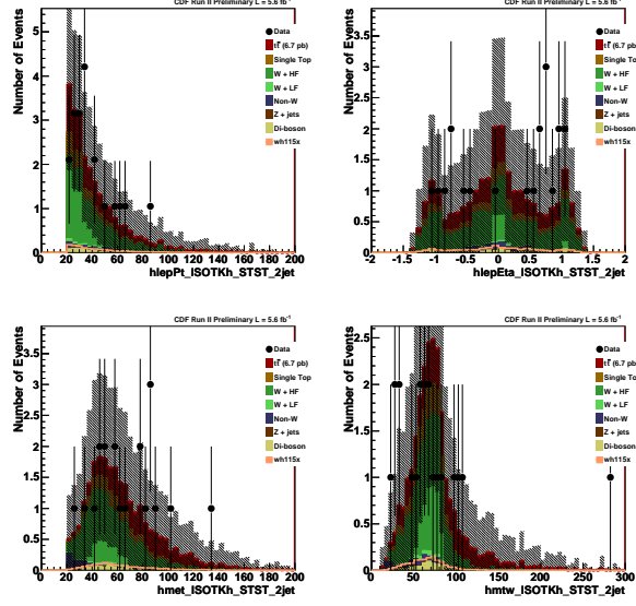
Figure 18: STST kinematic distributions for isolated track p_T , \eta , E_T , and W transverse mass.
