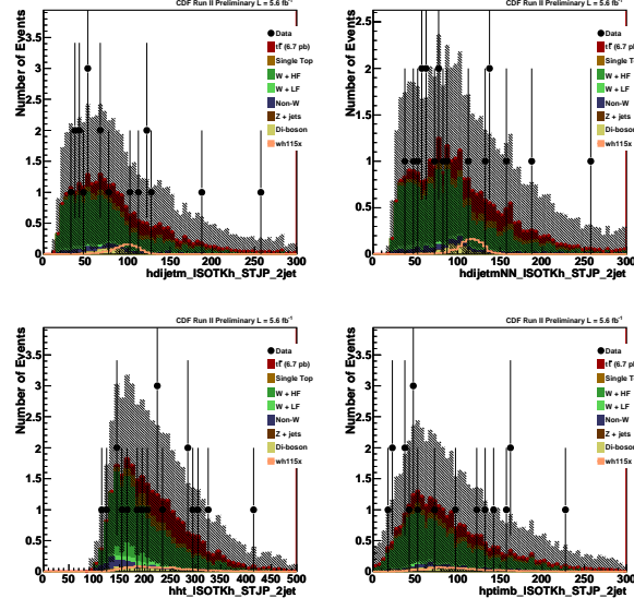
Figure 25: STJP kinematic distributions for dijet mass before and after bjet energy correction, H_T , and P_T imbalance.
