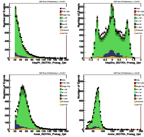
Figure 12: Pretag kinematic distributions for isolated track p_T , \eta , E_T , and W transverse mass.
