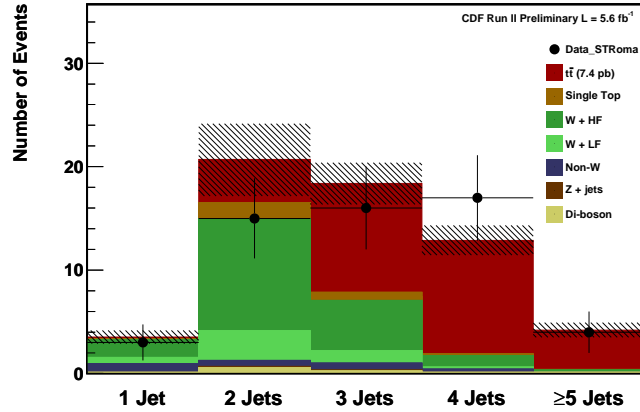
Figure 11: Number of expected and observed events for ST+RomaNN tag category.
