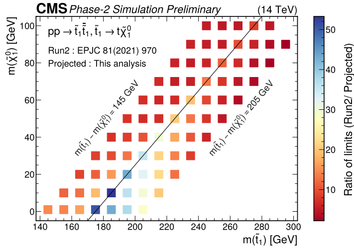
Figure 11: Ratio of expected 95% CL upper limits of the combined search for top squarks from Ref. [28] to the ones derived in the context of this search for the low top squark-neutralino mass plane. The center line corresponds to \Delta M(\tilde{t}_1, \tilde{\chi}_1^0) = 175 GeV.
