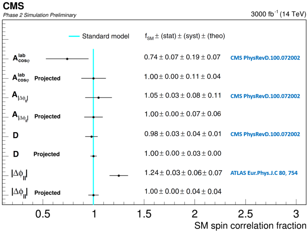
Figure 6: Extracted values of f_{SM} from laboratory-frame spin correlation variables by CMS [26] and ATLAS [27] at 13 TeV and projected values at 14 TeV. The measured and projected values with their statistical, systematic, and theoretical uncertainties are given on the right. Statistical uncertainties of the data on the projected values are smaller than 0.004 and hence, denoted with 0.00. As per Yellow Report recommendations theory uncertainties are reduced by 50% for projected values.
