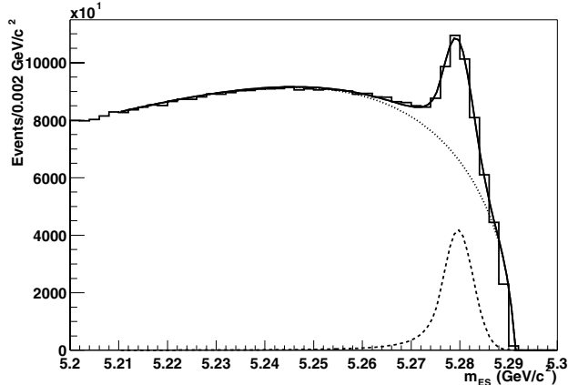
Figure 1: Distribution of the energy substituted mass m_{ES} in data for the fully reconstructed B mesons (histogram). The solid curve shows the result of the fit (see text). Also shown are the signal (dashed curve) and the background (dotted curve) components.
