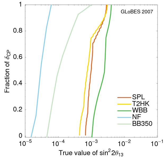
Figure 3a: (Color) Discovery reach for \theta_{13} .
