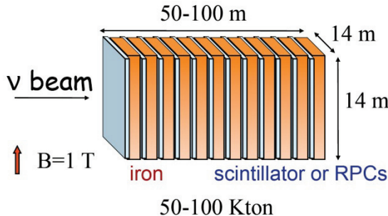
Figure 2: (Color) Schematic of the MIND concept for the
