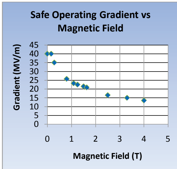
Figure 4: (Color) Maximum safe operating gradient v. magnetic field.
