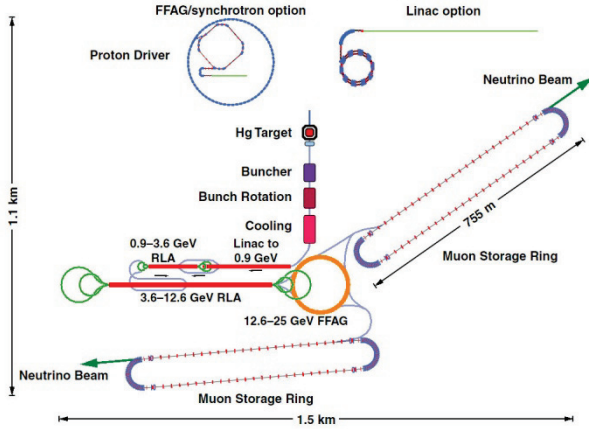
Figure 1: (Color) ISS Neutrino Factory facility baseline.
