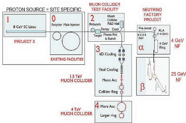
Figure 6: (Color) Muon Accelerator Complex “Vision” for Fermilab.
