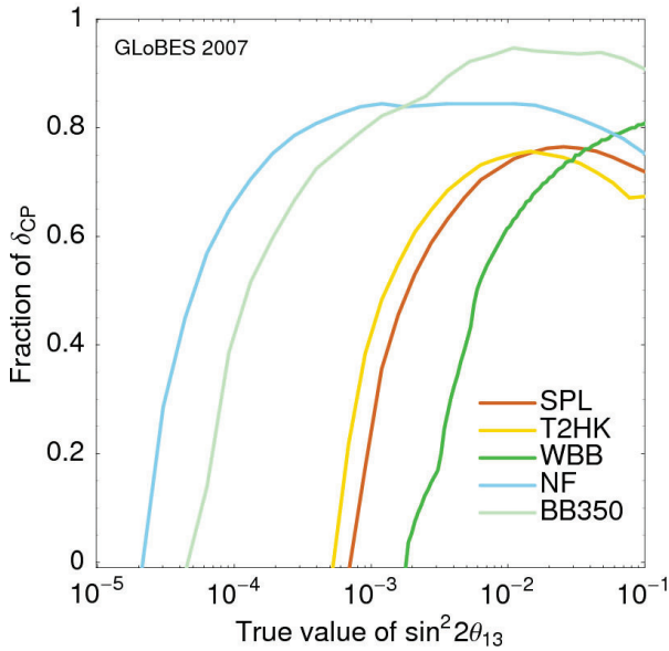
Figure 3c: (Color) Reach in the CP phase \delta .
