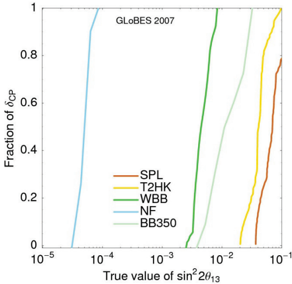
Figure 3a: (Color) Reach for determination of the mass hierarchy.
