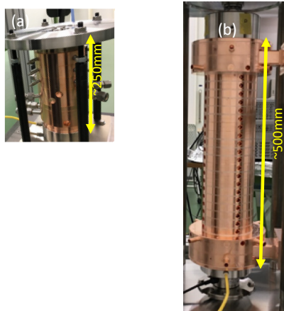
Figure 3: (a) laser-driven photocathode electron RF gun and (b) traveling wave buncher tube.
