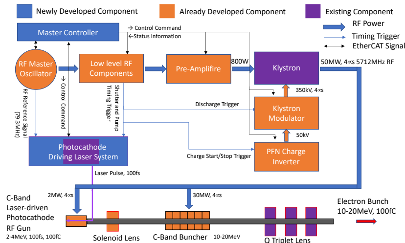
Figure 2: An outline of the linac with the precise synchronization between the RF and the laser pulses.
