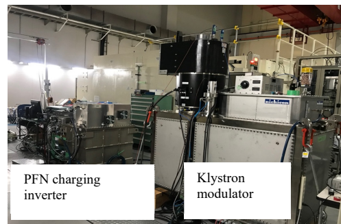
Figure 5: PFN charge inverter and klystron modulator during a high-power test.
