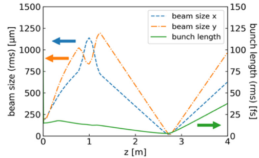
Figure 1: Transverse beam envelopes and a bunch length along the linac obtained by electron beam tracking simulations.
