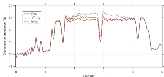
Figure 7: TDR measurements used for prototype stripline alignment, clearly identifying the location of the three Macor supports.
