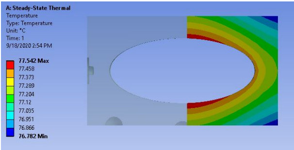
Figure 4: Thermal modeling of the ceramic chamber with 100 W of power dissipation. Ducting routes air from fans on the cover to cool the ceramic chamber and the ferrites.
