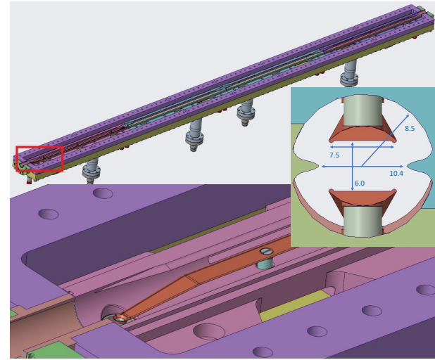
Figure 5: Swap-out kicker 4-module assembly (top), stripline dielectric support and taper (bottom), and transverse section with dimensions in mm (insert).
