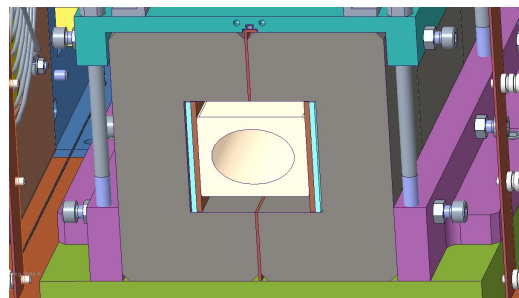
Figure 2: BTA ferrite-loaded kicker cross section.
