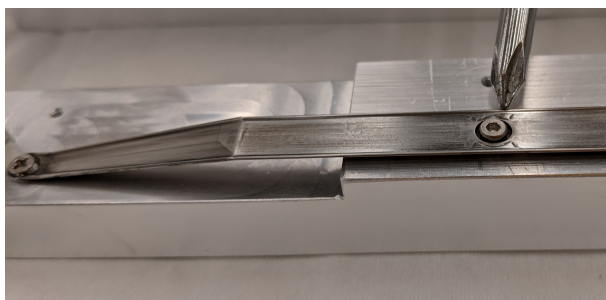
Figure 8: Tapered end of a prototype molybdenum stripline electrode which was fabricated at LBNL.
