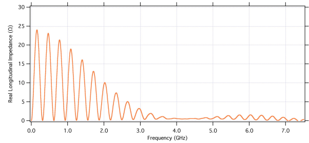
Figure 6: Real longitudinal impedance of the tapered stripline kicker.
