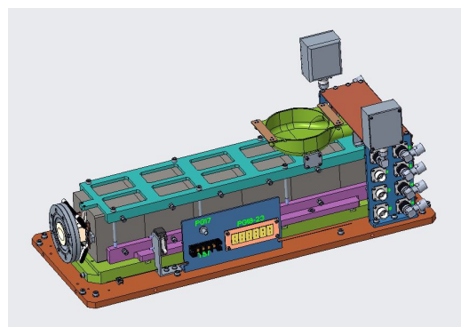
Figure 3: BTA ferrite-loaded kicker assembly without the cover.
