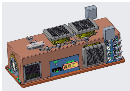
Figure 1: Complete BTA ferrite-loaded kicker assembly.
