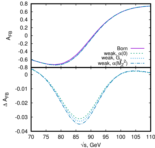
Fig. 2. The A_{FB} asymmetry and \Delta A_{FB} in the Born and 1-loop EW approximations within the \alpha(0) , G_\mu , and \alpha(M_Z^2) EW schemes versus the c.m.s. energy.
