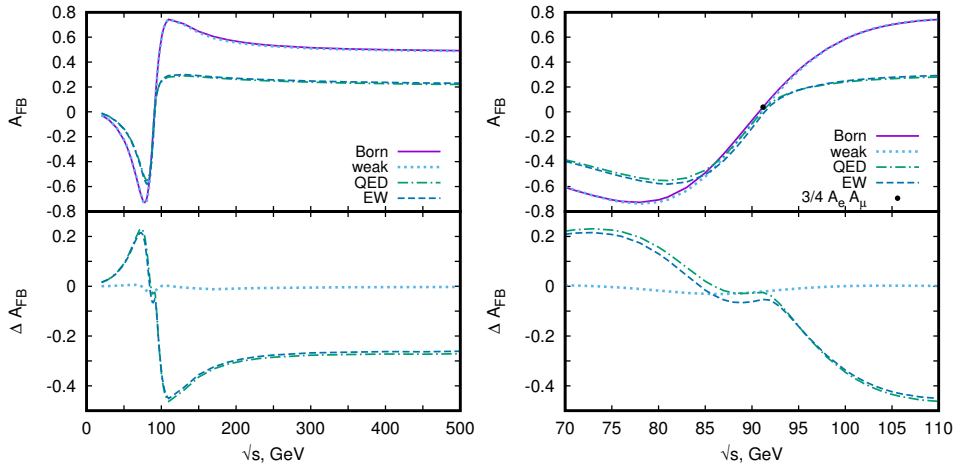
Fig. 1. The A_{FB} asymmetry at the Born and 1-loop (weak, QED, EW) levels and the corresponding shifts \Delta A_{FB} for a wide c.m.s. energy range (left) and for the Z -peak region (right).
