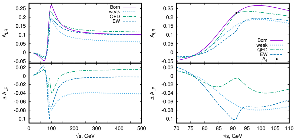
Fig. 3. The A_{\text{LR}} asymmetry in the Born and 1-loop (weak, pure quantum electrodynamics (QED), and electroweak (EW)) approximations and \Delta A_{\text{LR}} versus c.m.s. energy in a wide range (left) and for the Z -peak region (right).
