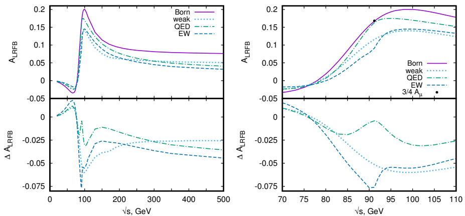
Fig. 4. The A_{\text{LRFB}} asymmetry in the Born and 1-loop (weak, QED, EW) approximations and \Delta A_{\text{LRFB}} for c.m.s. energy range (left) and for the Z -peak region (right).
