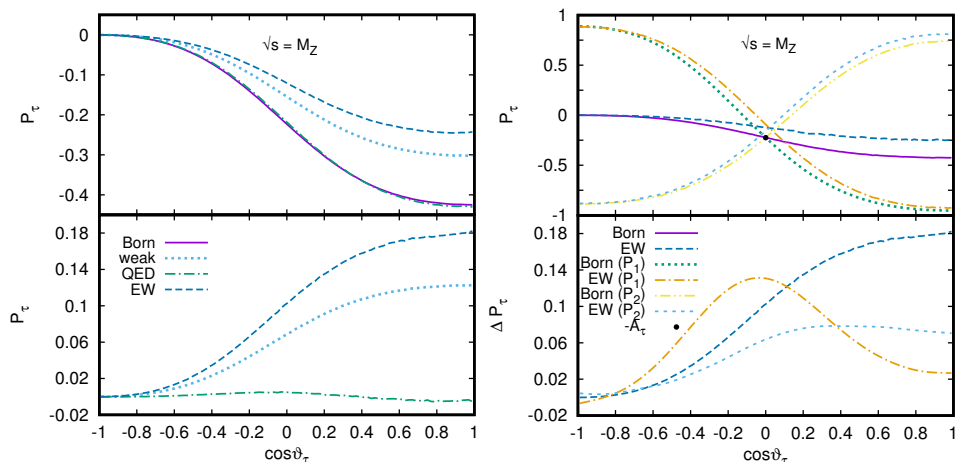
Fig. 5. P_\tau polarization in the Born and 1-loop (weak, pure QED, and EW) approximations as a function of \cos\vartheta_\tau at \sqrt{s} = M_Z (left), P_\tau polarization for unpolarized and polarized cases with P_1 = (-0.8, 0.3) and P_2 = (0.8, -0.3) degrees of initial beam polarizations in the Born and EW 1-loop approximations versus cosine of the final \tau lepton angle (right).
