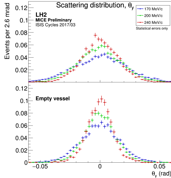
Figure 6: Distribution of \theta_y for the three momenta settings. For vessel full (top) and empty (bottom) configurations.
