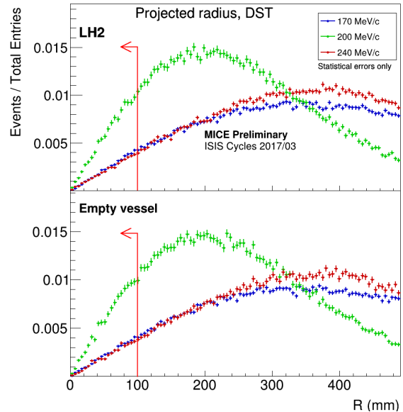
Figure 3: Particles with projected R = \sqrt{x^2 + y^2} > 100 mm at the final station of the DS tracker are rejected.
