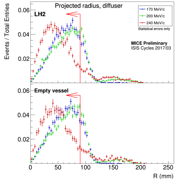
Figure 2: Particles with projected R = \sqrt{x^2 + y^2} > 90 mm at the position of the diffuser are rejected.
