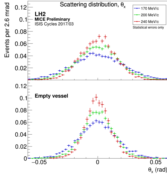
Figure 5: Distribution of \theta_x for the three momenta settings. For vessel full (top) and empty (bottom) configurations.
