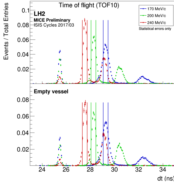
Figure 4: Time-of-flight distribution with selection intervals.
