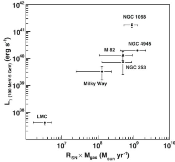
Figure 4.3: Plot of SN rate multiplied by total gas mass against \gamma -ray luminosity for NGC 1068, NGC 4945, NGC 253, M 82, the LMC and the Milky Way. Taken from Lenain et al. (2010).
