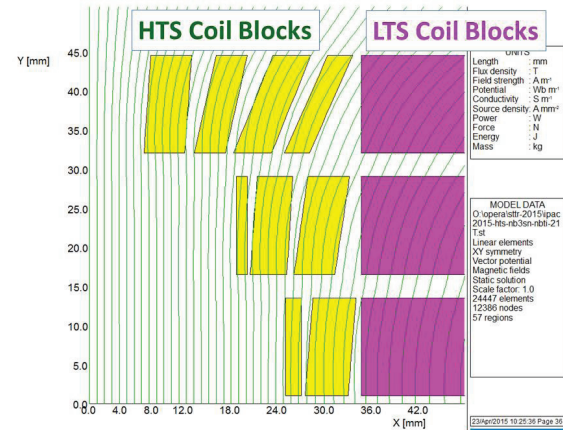
Figure 3: HTS (yellow, lighter shade) and LTS (pink, darker shade) coil blocks. HTS coil blocks are optimized to be parallel the field lines in a 50 mm aperture dipole.
