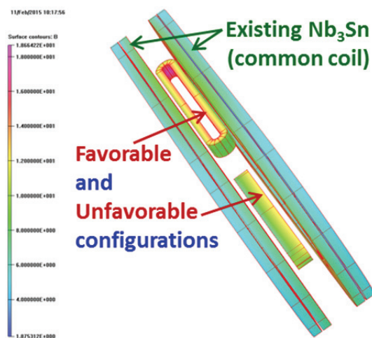
Figure 6: Simplified magnetic model (only coils shown) of two set of HTS insert coils placed between Nb 3 Sn coils of magnet DCC017.
