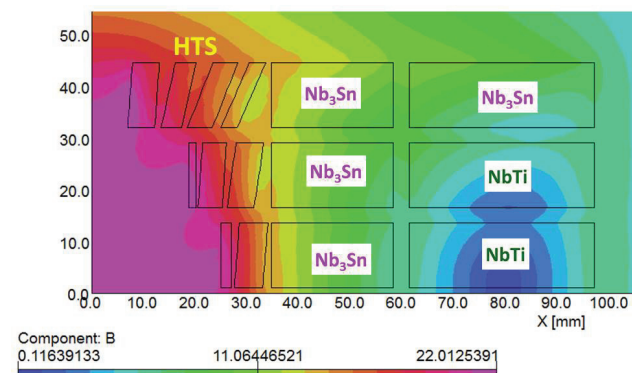
Figure 2: Field contours at central field of 21 T. Blocks with x < 35 mm use HTS (ReBCO tape); those with x > 35 mm use Nb 3 Sn or NbTi (LTS).
