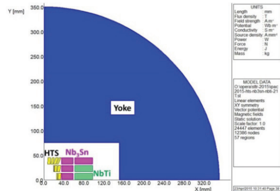
Figure 1: Quadrant of the magnetic model consisting of HTS, Nb 3 Sn and NbTi (LTS) coil blocks and iron yoke.
