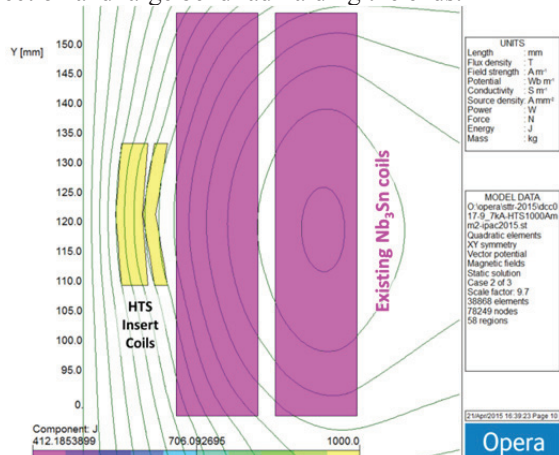
Figure 5: Field lines in one half of one aperture in the proof-of-principle dipole. HTS tape coil blocks (yellow, light shade), are aligned with the field lines and inserted within the aperture of the Nb 3 Sn coils (pink, darker).
