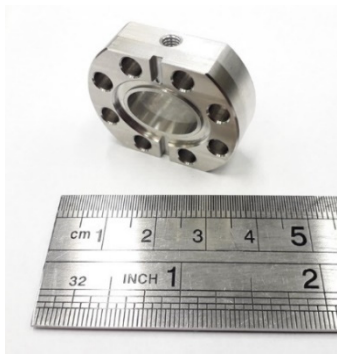
Figure 7: The vacuum flange developed for the aluminium vacuum chamber.
