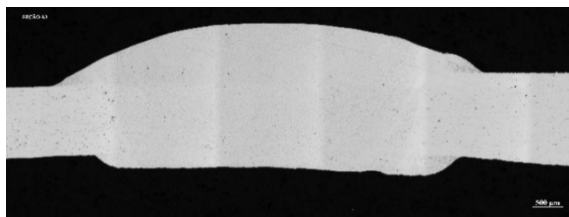
Figure 9: Metallography analysis indicating 0,2% porosity.
