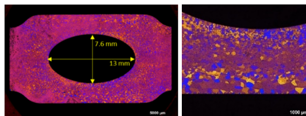
Figure 2: Metallographic image from the central part of chamber's cross section.
