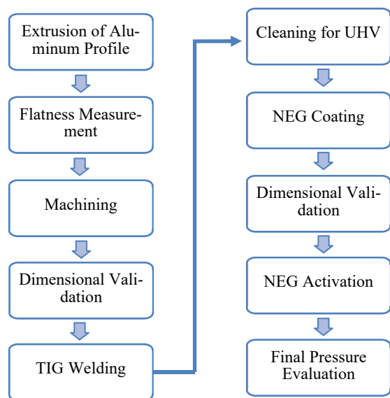
Figure 4: Sequence of processes to fabricate a complete chamber.
