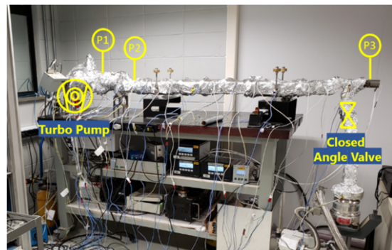
Figure 10: Set up for NEG activation tests.
