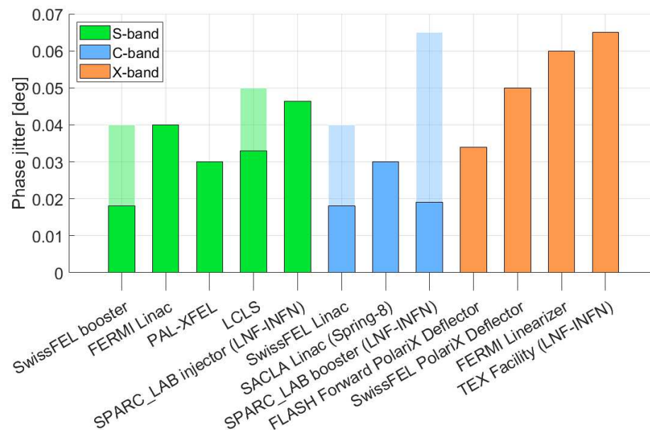
Figure 1. The state of the art for measured phase stability in pulsed RF plants worldwide is compared with the facilities at LNF-INFN. The solid fill color represents the best results published or disseminated by other laboratories, while the transparent fill color accounts for the spread between the worst- and best-case scenarios when multiple plants are available.
