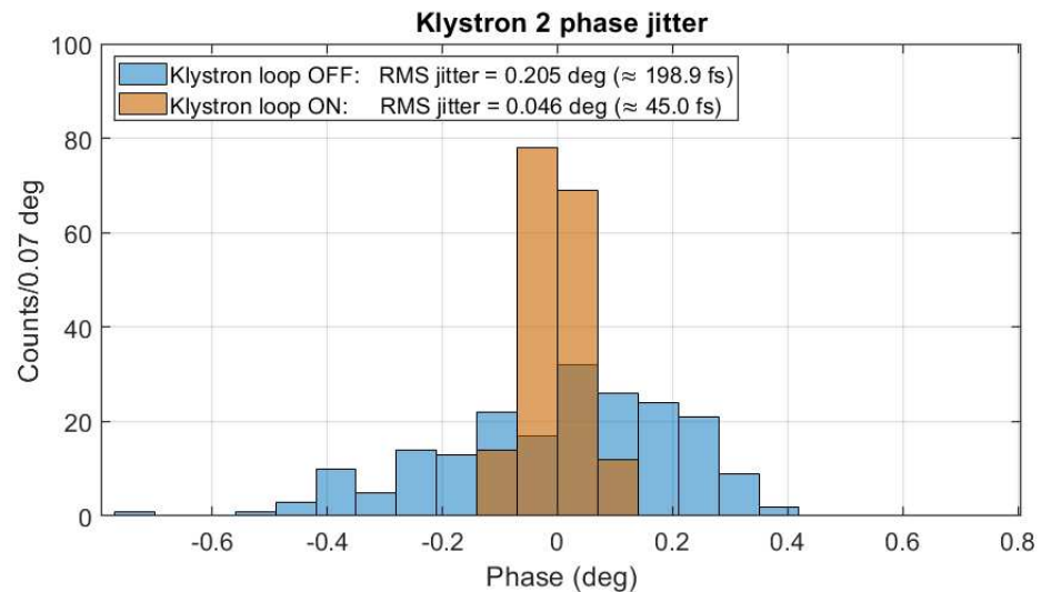
Figure 3. Recent measurement at SPARC_LAB of the S-band fast intra-pulse feedback capability with Libera LLRF front-end. The klystron phase measured with feedback off is shown in blue, whereas that with feedback on is shown in orange. There are approximately 200 shots at 10 Hz repetition rate. A jitter reduction down to 0.046 deg RMS has been obtained, with an overall compression of a factor >4 .
