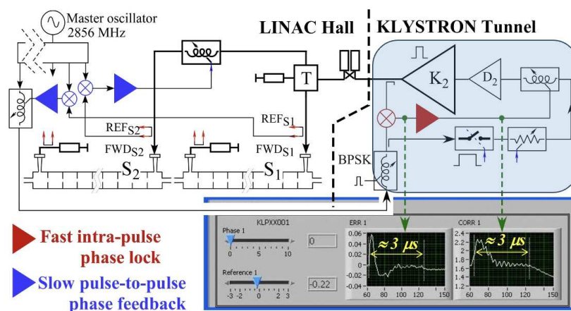
Figure 2. SPARC_LAB klystron n.2 (K2) RF system. Highlighted block diagram of the fast intra-pulse feedback that includes the solid state driver amplifier (D2) and the Binary Phase Shift Keying (BPSK), which realizes the phase jump for the pulse compressor that feeds the two accelerating sections (S1 and S2). Moreover, a screenshot of its control system with the typical phase detector and error amplifier output signals is reported at the bottom.
