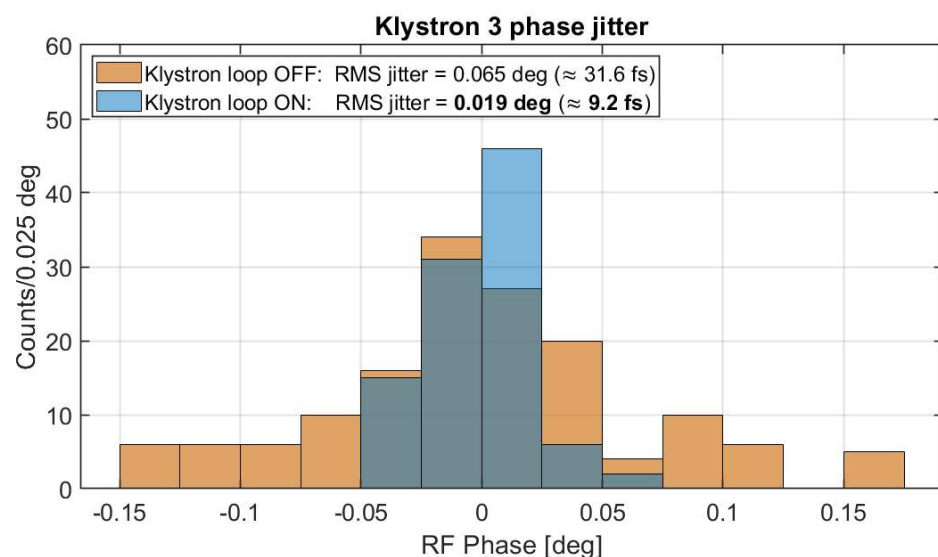
Figure 6. Intra-pulse feedback prototype measurement results at SPARC_LAB facility on the C-band power plant. In bold the results obtained with the new feedback on.
