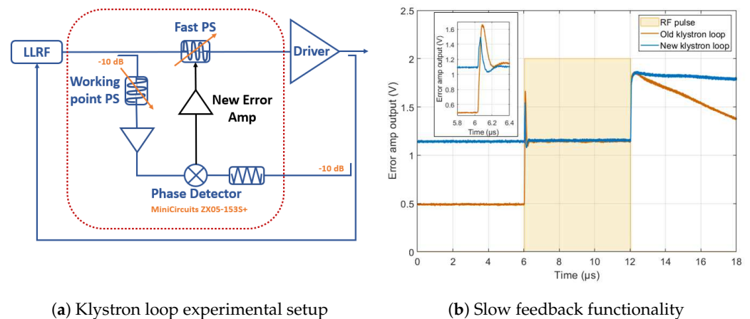
Figure 5. (a) Block diagram of the laboratory experimental setup for the klystron loop bench test, and (b) oscilloscope capture of the functionality of the slow feedback. The error amplifier output without slow feedback is shown in orange; the same output with slow feedback in operation is shown in blue. It can be clearly seen that the loop also allows us to reach a phase value close to the desired one when the RF pulse is off. This minimizes the transient and the overall phase modulation required to reach the steady state, as shown in the waveform zoom.
