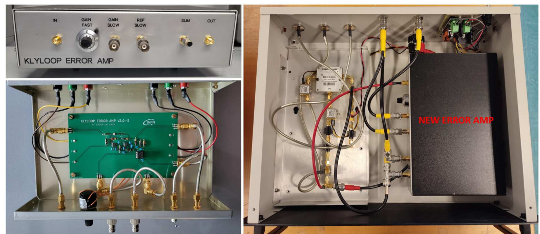
Figure 4. New error amplifier board ( left ) and the new RF chassis ( right ) realized at INFN-LNF laboratories for the klystron loop upgrade.
